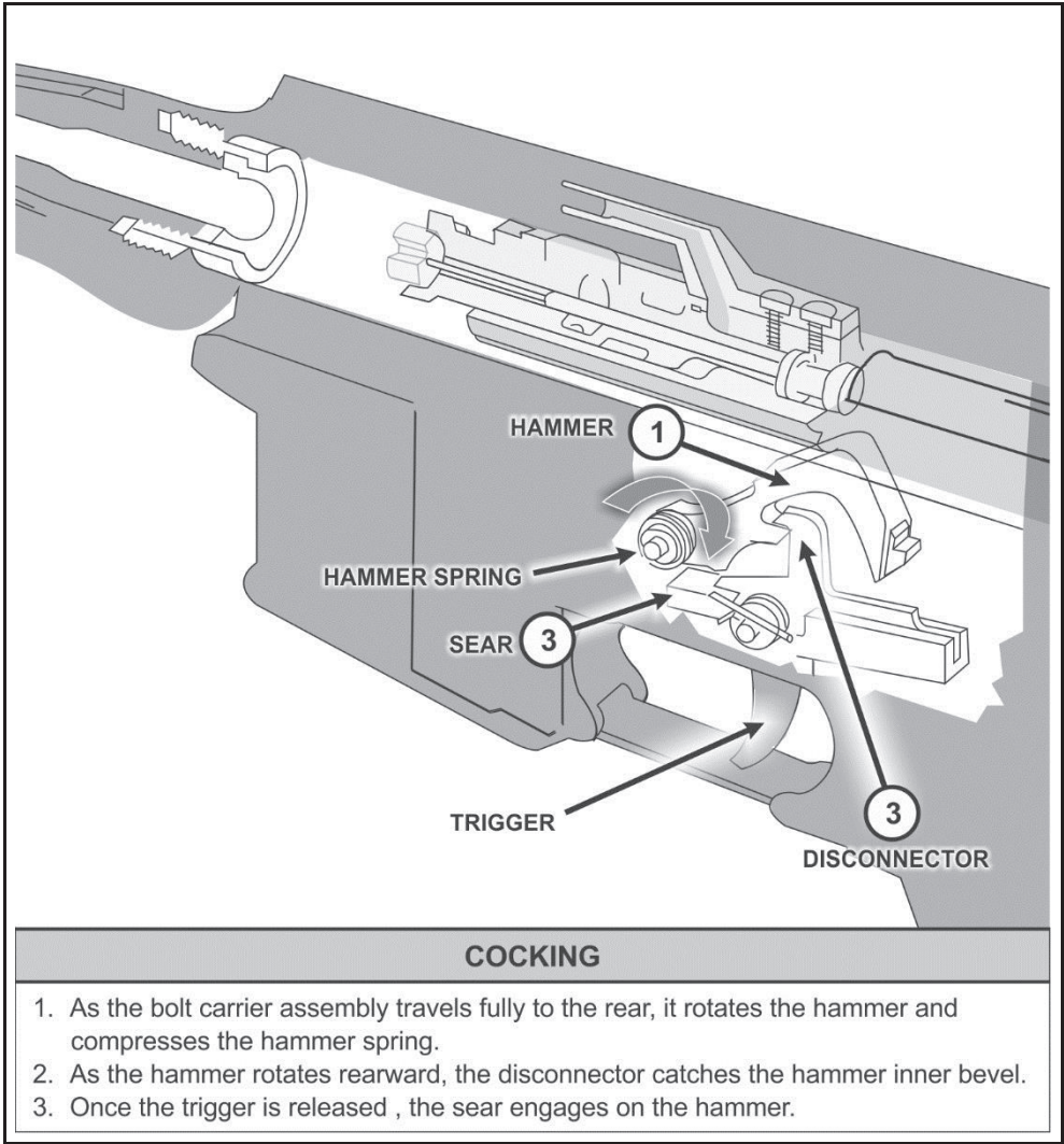
Figure 2-10. Cocking example
