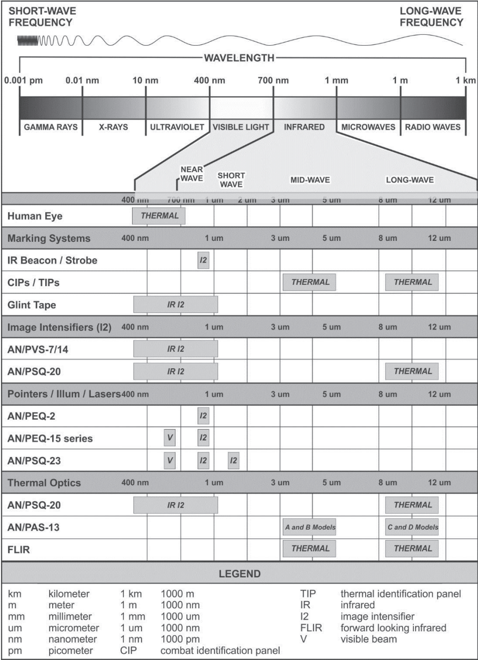
Figure 3-5. Electromagnetic spectrum
