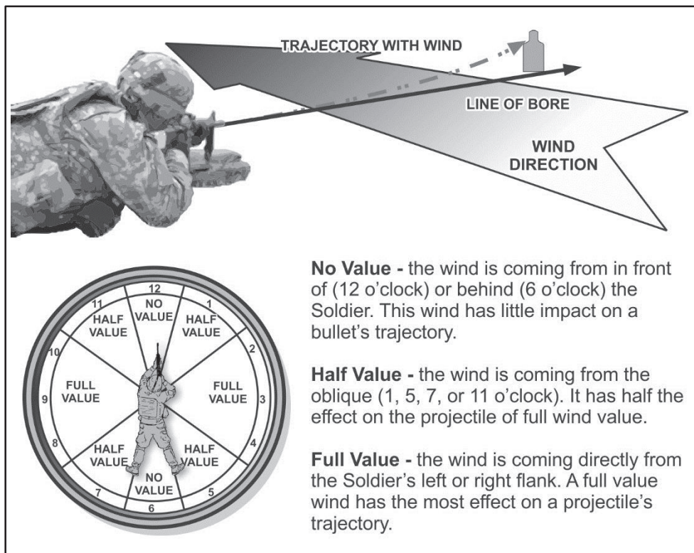
Figure 7-11. Wind effects
