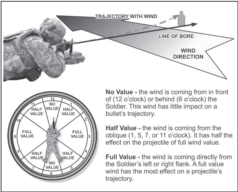
Figure C-9. Wind effects
