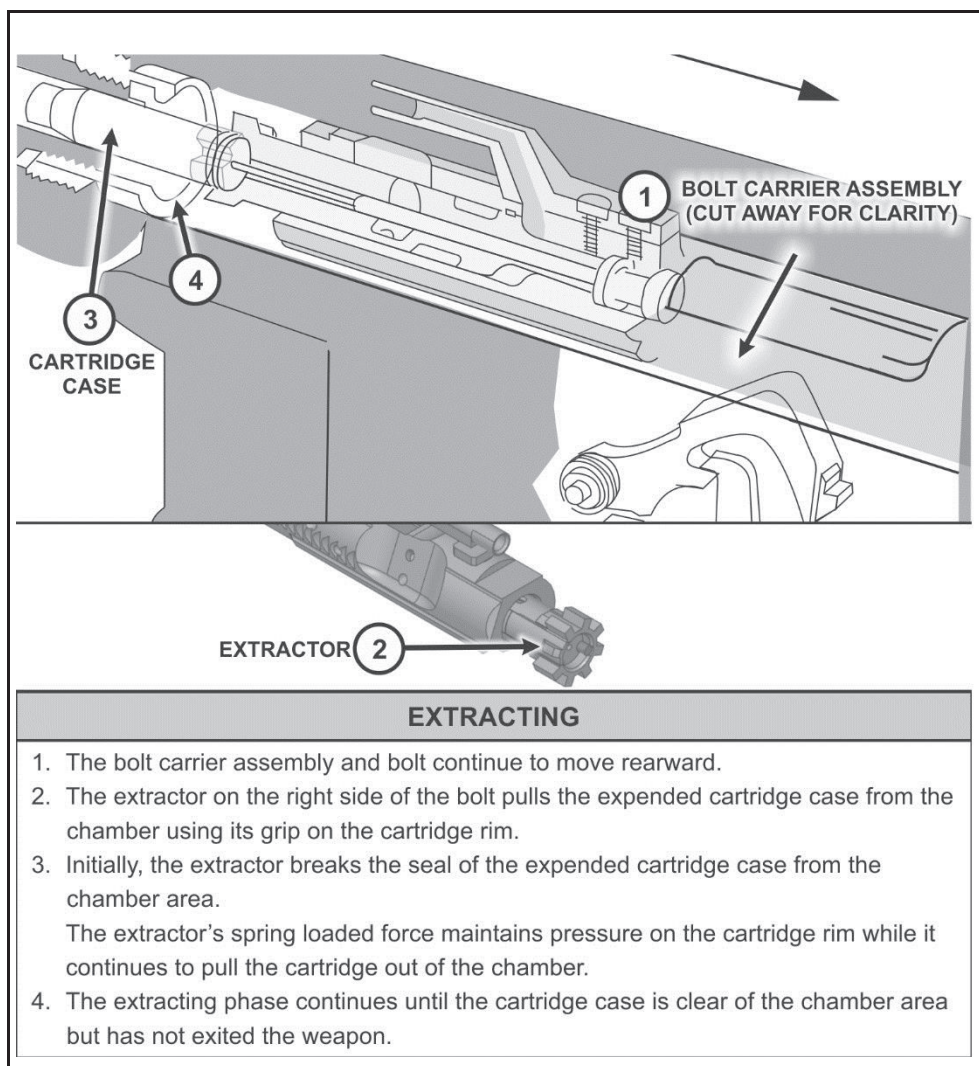
Figure 2-8. Extraction example
