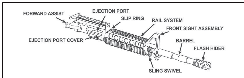
Figure 2-1. Upper receiver
