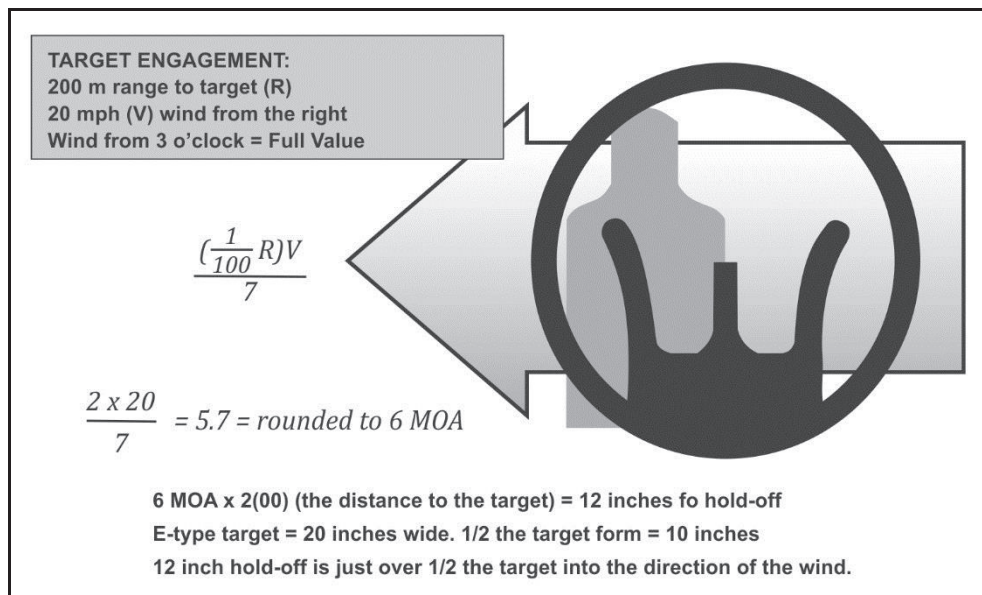
Figure C-11. Hold-off example
