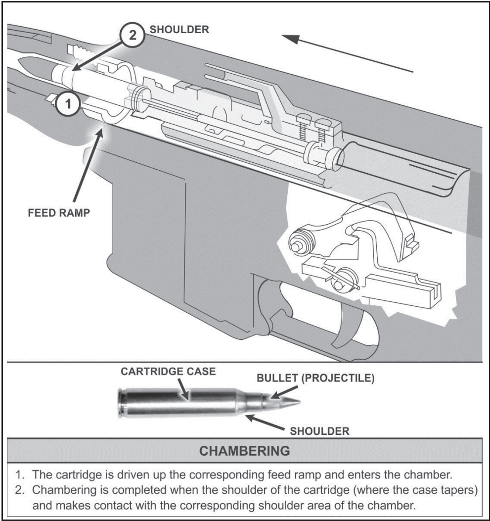
Figure 2-4. Chambering example
