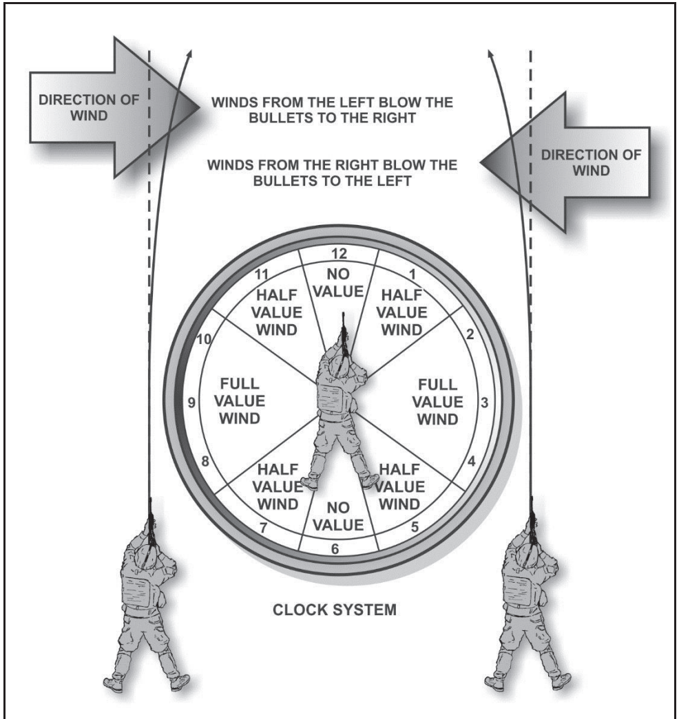
Figure C-8. Wind value
