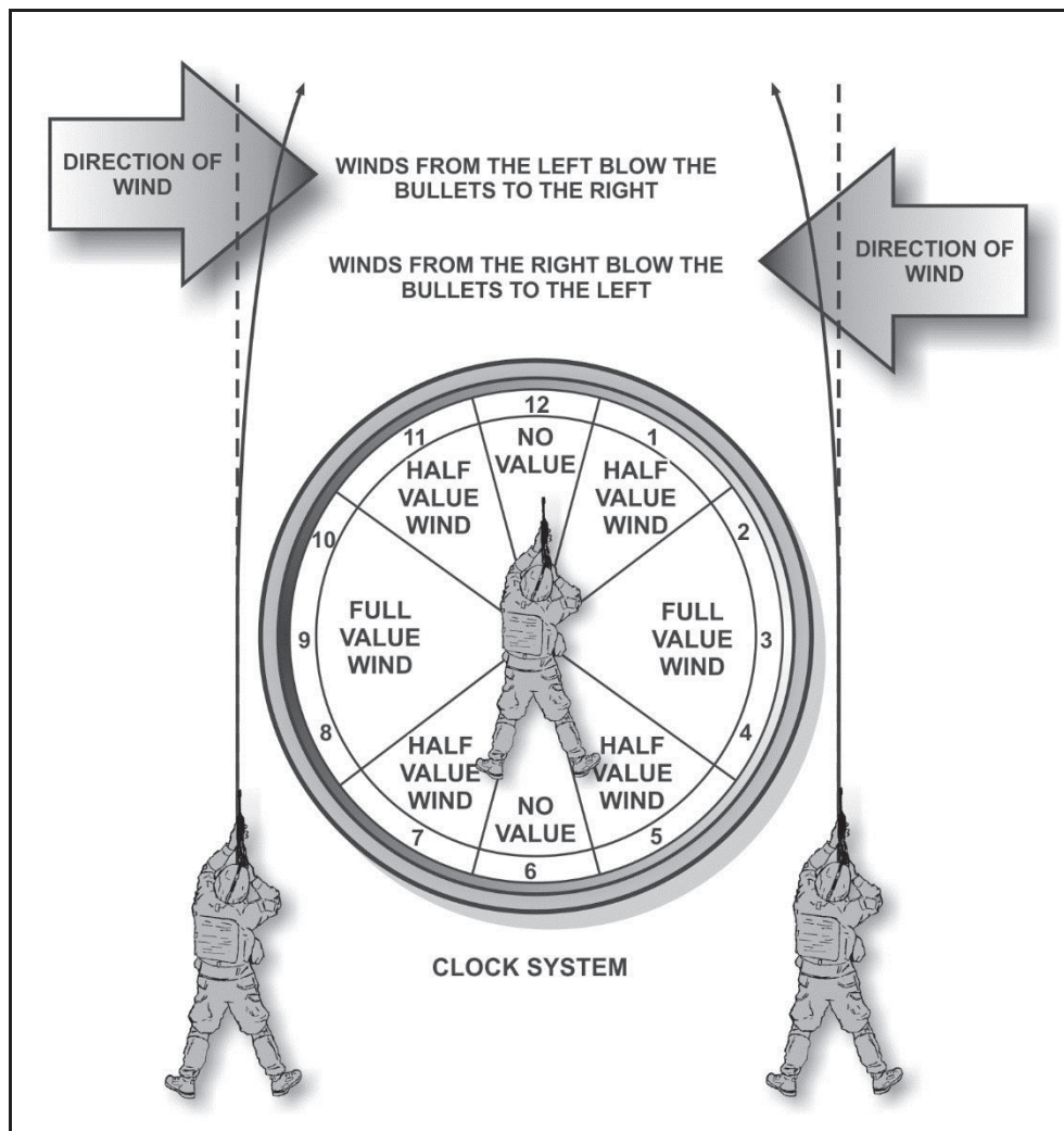
Figure 7-10. Wind value
