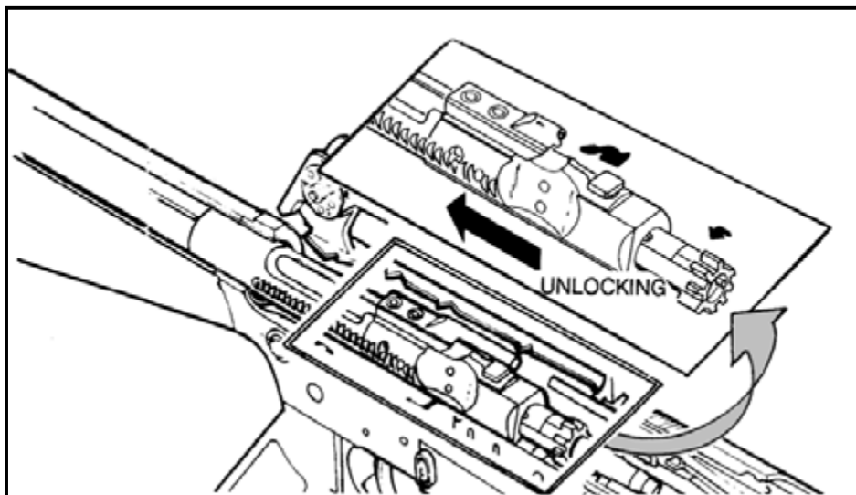
Figure 4-7. Unlocking.
