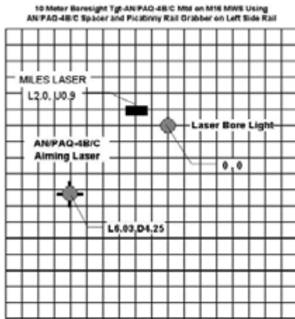
10 Meter Bore Sight Target for 300m Zero (13 Dec 99)
