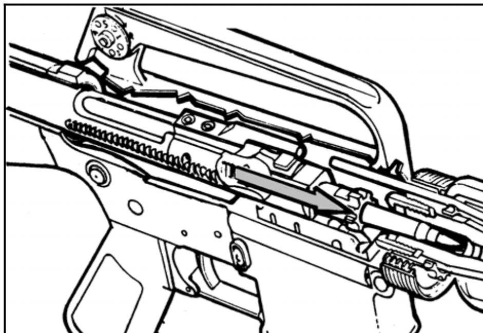
Figure 4-4. Chambering.
