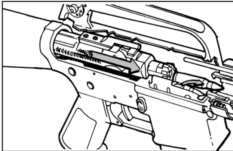
Figure 4-3. Feeding.
