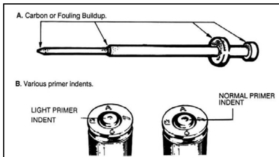
Figure 3-2. Failure to fire.
