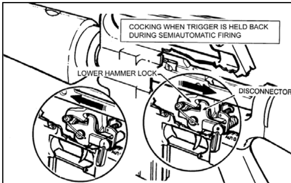
Figure 4-10. Cocking.
