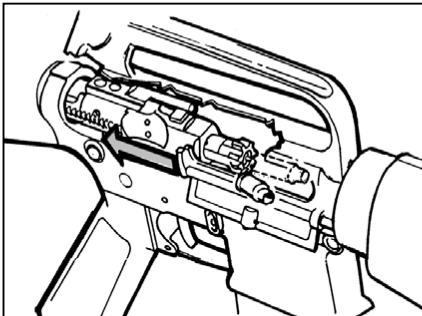
Figure 4-9. Ejecting.
