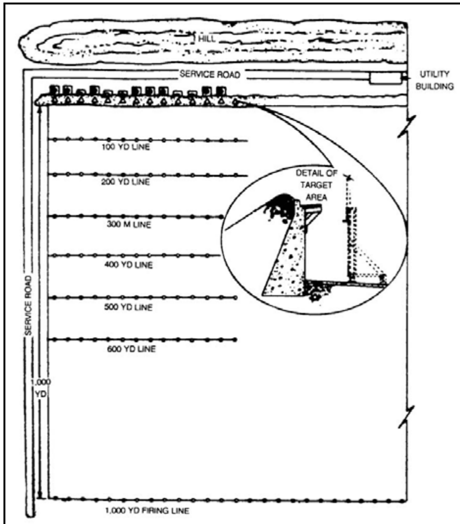
Figure 5-24. Known-distance range.
