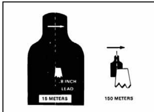
Figure 7-30. Lead increasing at greater ranges.
