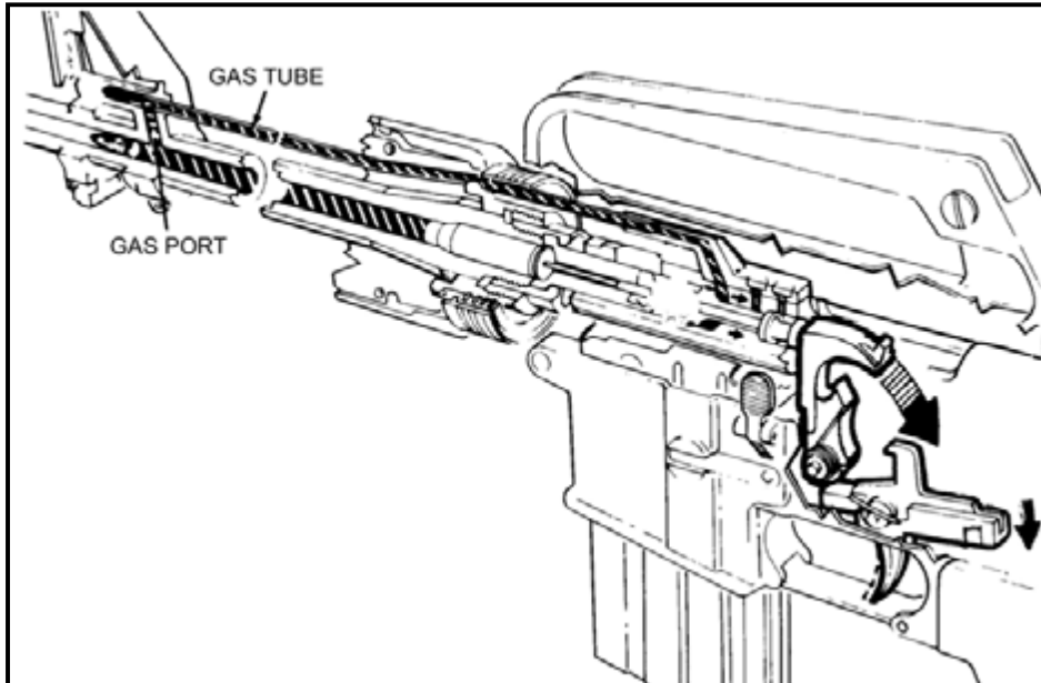
Figure 4-6. Firing.
