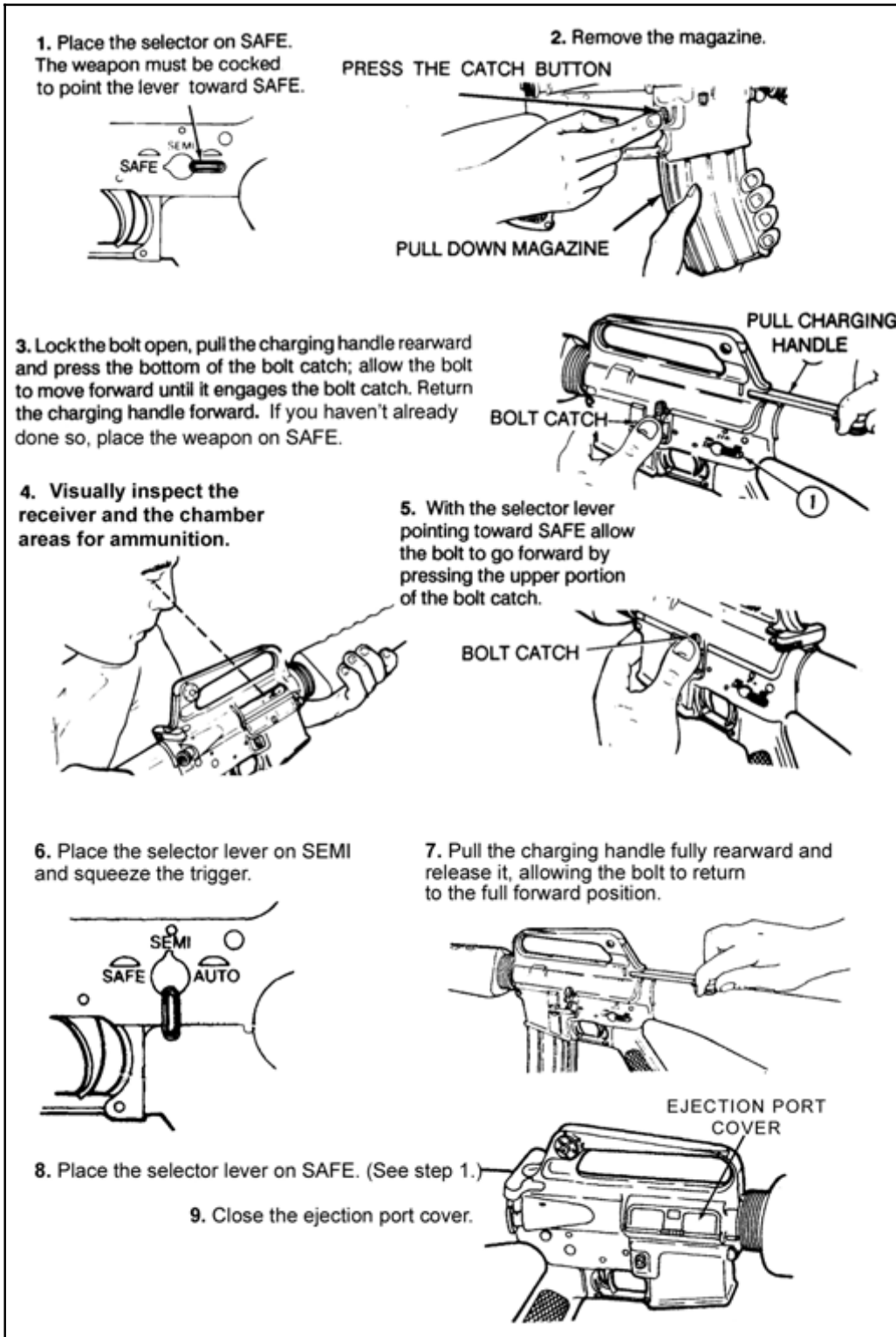
*Figure 4-2. Clearing.
