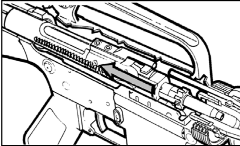
Figure 4-8. Extracting.
