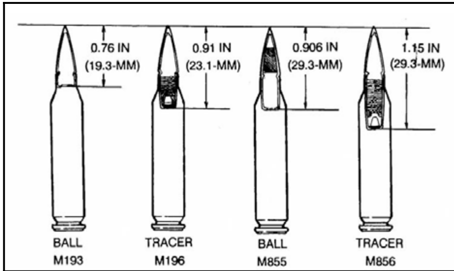
Figure 5-32. Projectile differences.
