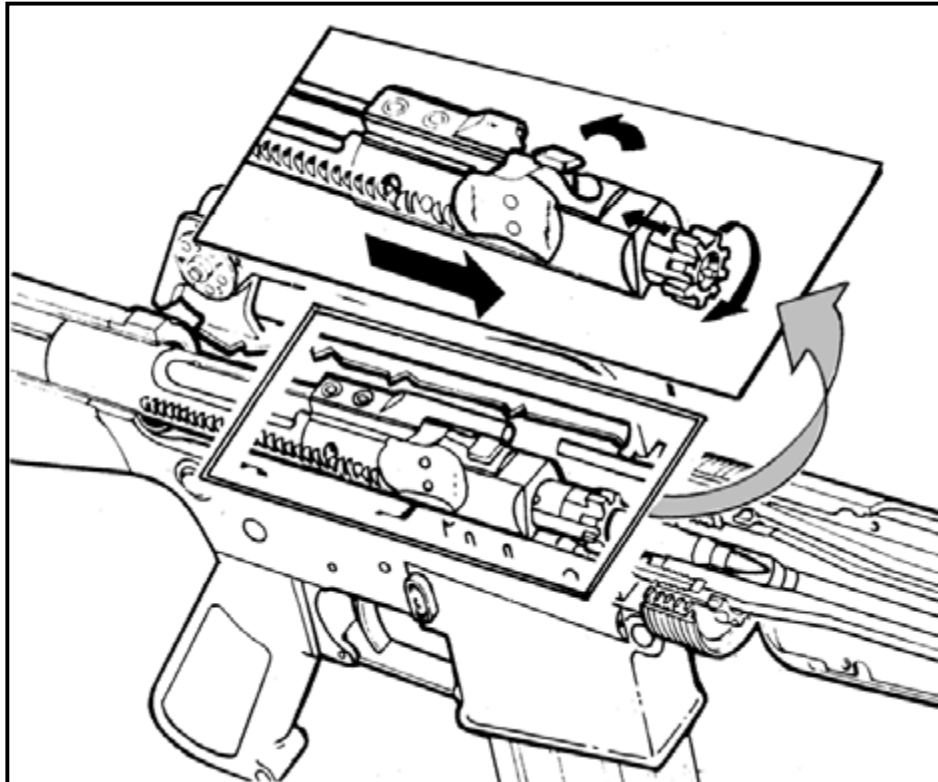
Figure 4-5. Locking.
