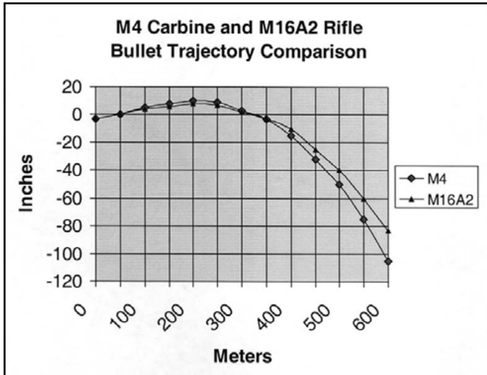
Figure 7-39. Bullet trajectory comparison.
