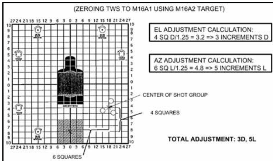
*Figure 8-10. Example of TWS zeroing adjustments.
