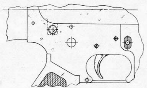
VIEW SHOWING MAGAZINE RELEASE
