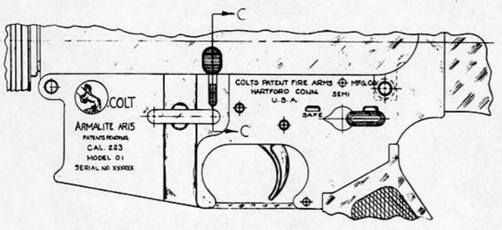
VIEW SHOWING SAFETY AND BOLT CATCH
