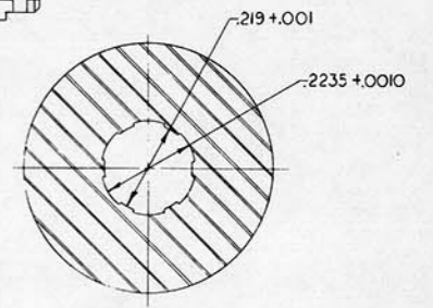
VIEW SHOWING RIFLING
