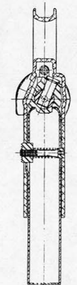
SECTION E-E THRU BOLT CAM AND MAGAZINE RELEASE
