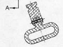
SECTION D-D THRU SLING
