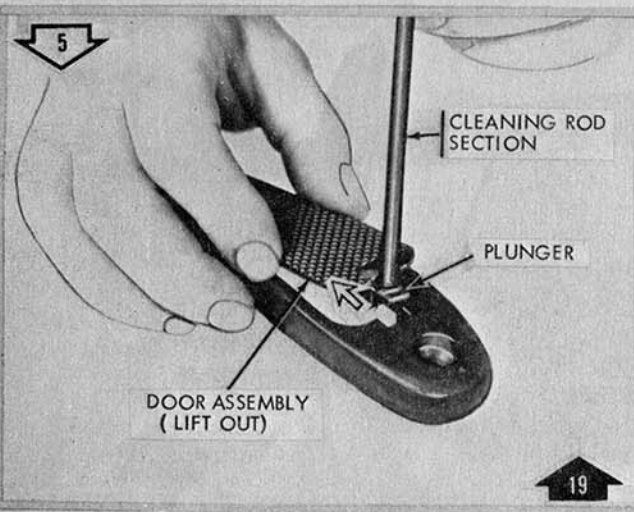
Unlock/Lock plunger and Remove/Install door assembly
