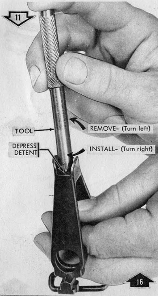
Remove/Install front sight post
