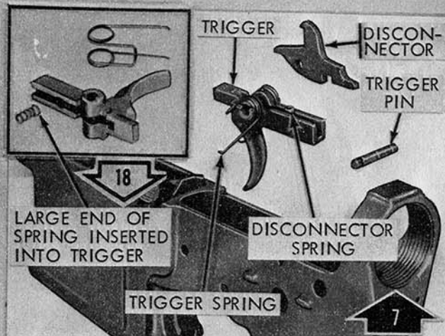
Remove/Install trigger, trigger spring, disconnecter, and disconnecter spring.
