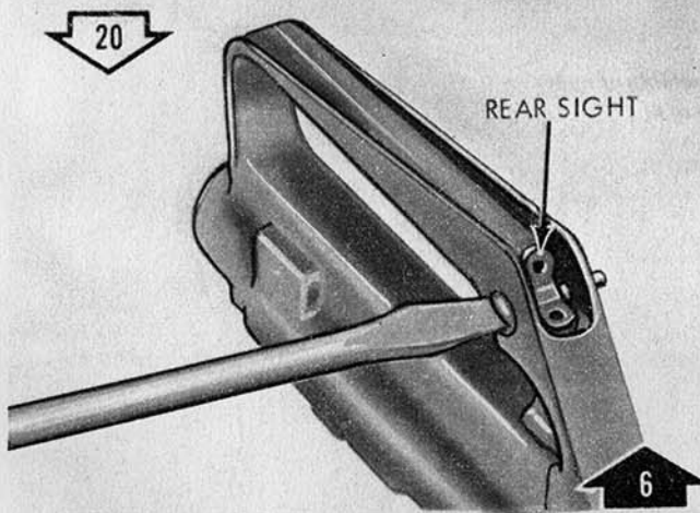
20 REAR SIGHT 6 Remove/Install rear sight windage screw.
