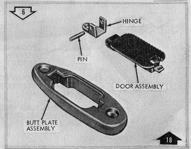
Remove/Install pivot latch pin and hinge.
