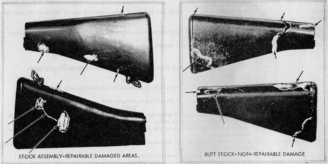
Figure 3-9. Repairable/non-repairable stock assemblies.
