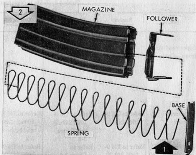
Remove/Install magazine spring and follower.
