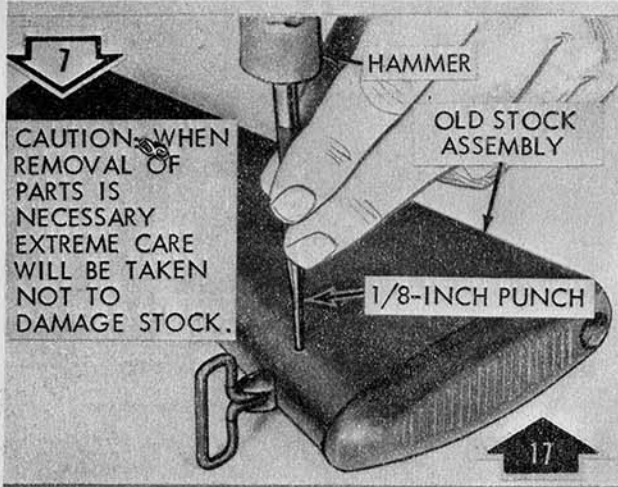
Remove/Install rear swivel spring pin.
