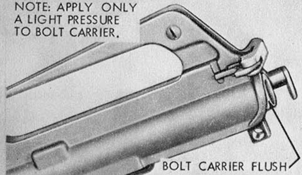
3. Incorrect headspace.
