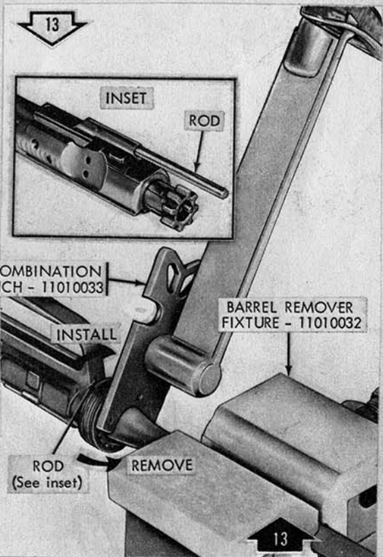
Remove/Install barrel nut assembly.
