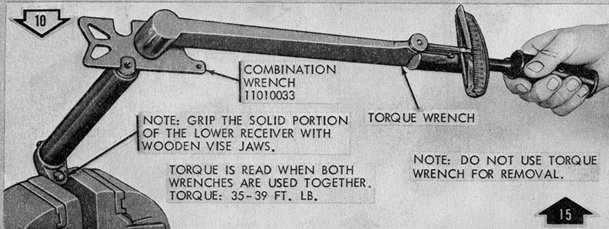
Loosen/Tighten lower receiver extension.
