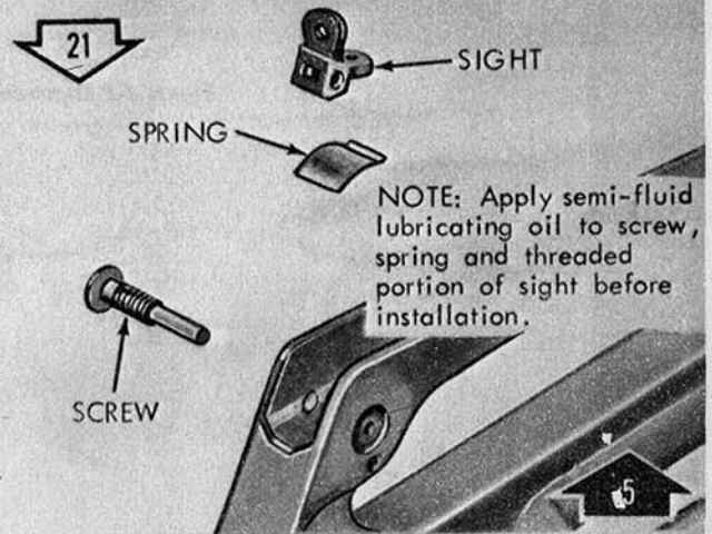
21 SIGHT SPRING SCREW 5 NOTE: Apply semi-fluid lubricating oil to screw, spring and threaded portion of sight before installation. Remove/Install rear sight and rear sight spring.
