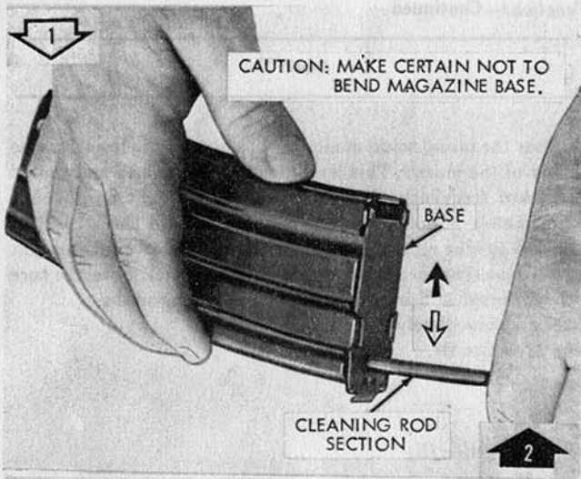
Remove/Install magazine base.
