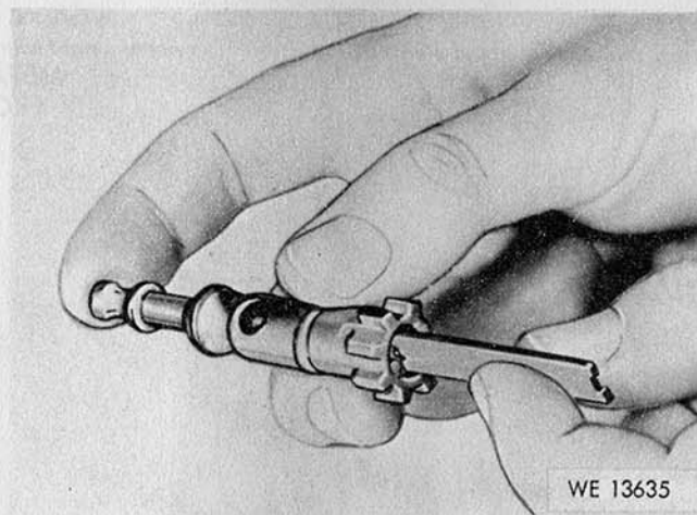
Figure 3-15. Check bolt with firing pin protrusion gage.
