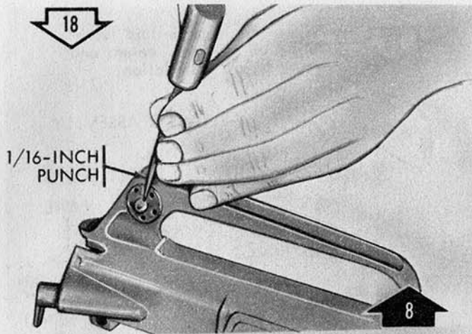
18 1/16-INCH PUNCH 8 Remove/Install rear sight windage drum spring pin.
