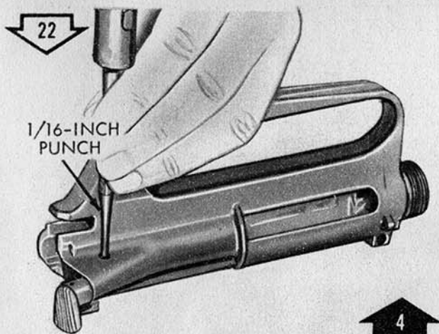
22 1/16-INCH PUNCH 4 Remove/Install spring pin.
