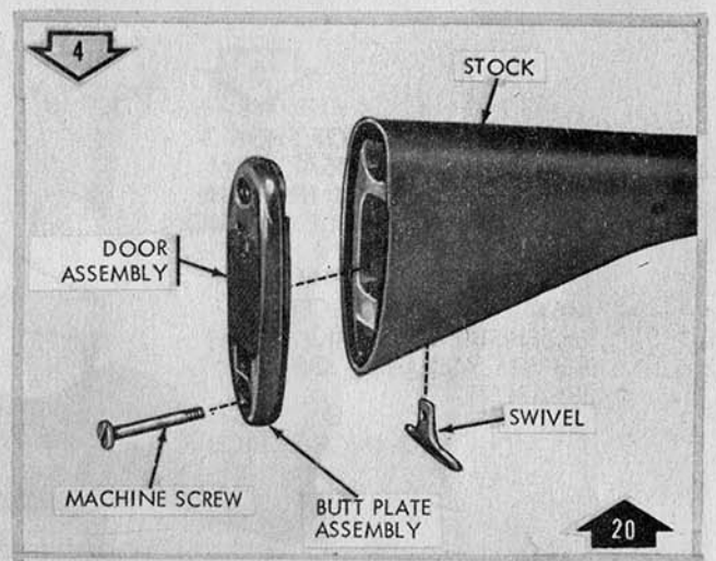
Remove/Install sling swivel, butt plate assembly and door assembly.
