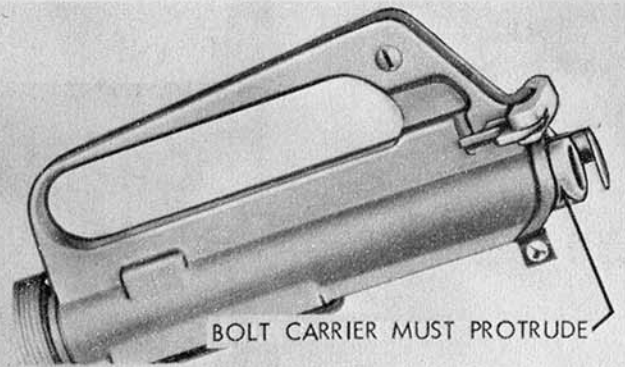
2. Correct headspace.
