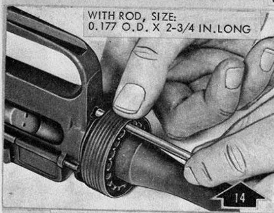
Install and align barrel nut assembly
