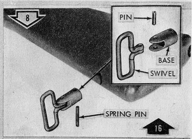
Remove/Install spring pin, gun sling swivel and base.
