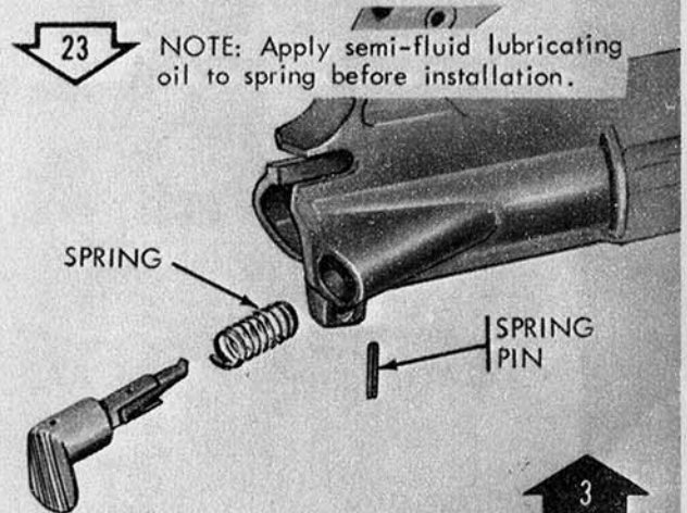
23 3 NOTE: Apply semi-fluid lubricating oil to spring before installation. Remove/Install forward assist assembly.
