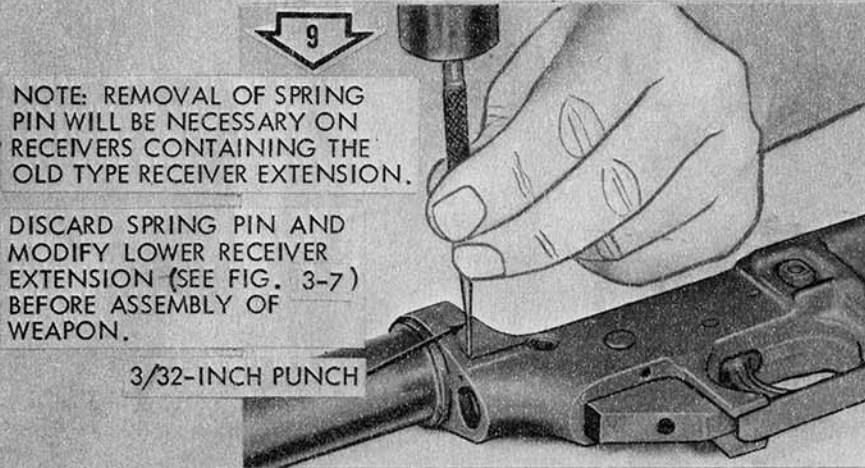
Remove lower receiver extension spring pin.
