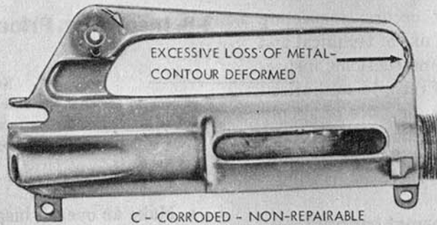
Figure 3-10. Repairable and non-repairable upper receivers—right side view.
