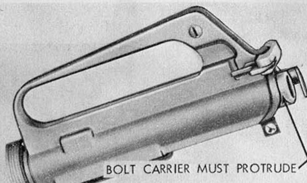
2. Correct headspace.
