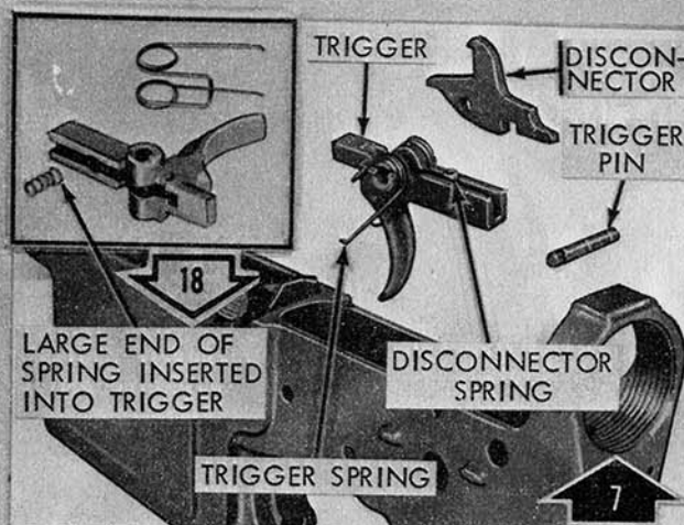
Remove/Install trigger, trigger spring, disconnecter, and disconnecter spring.
