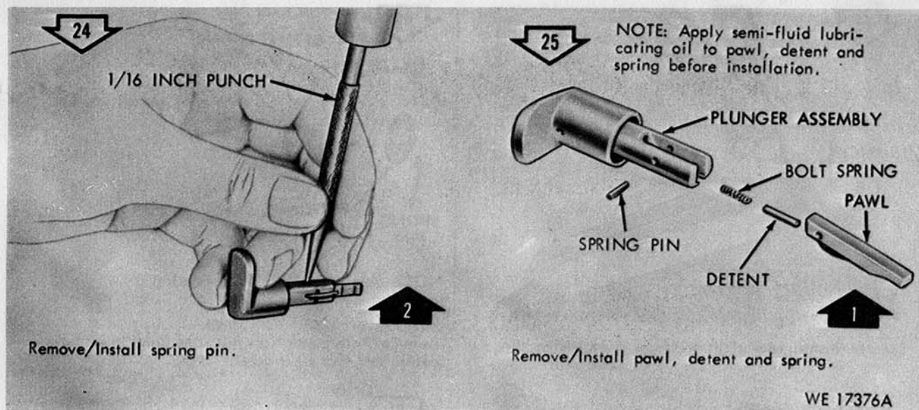
Figure 3-2. Disassembly/assembly of upper receiver group. (6 of 6)
