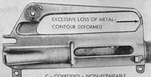
C - CORRODED - NON-REPAIRABLE
