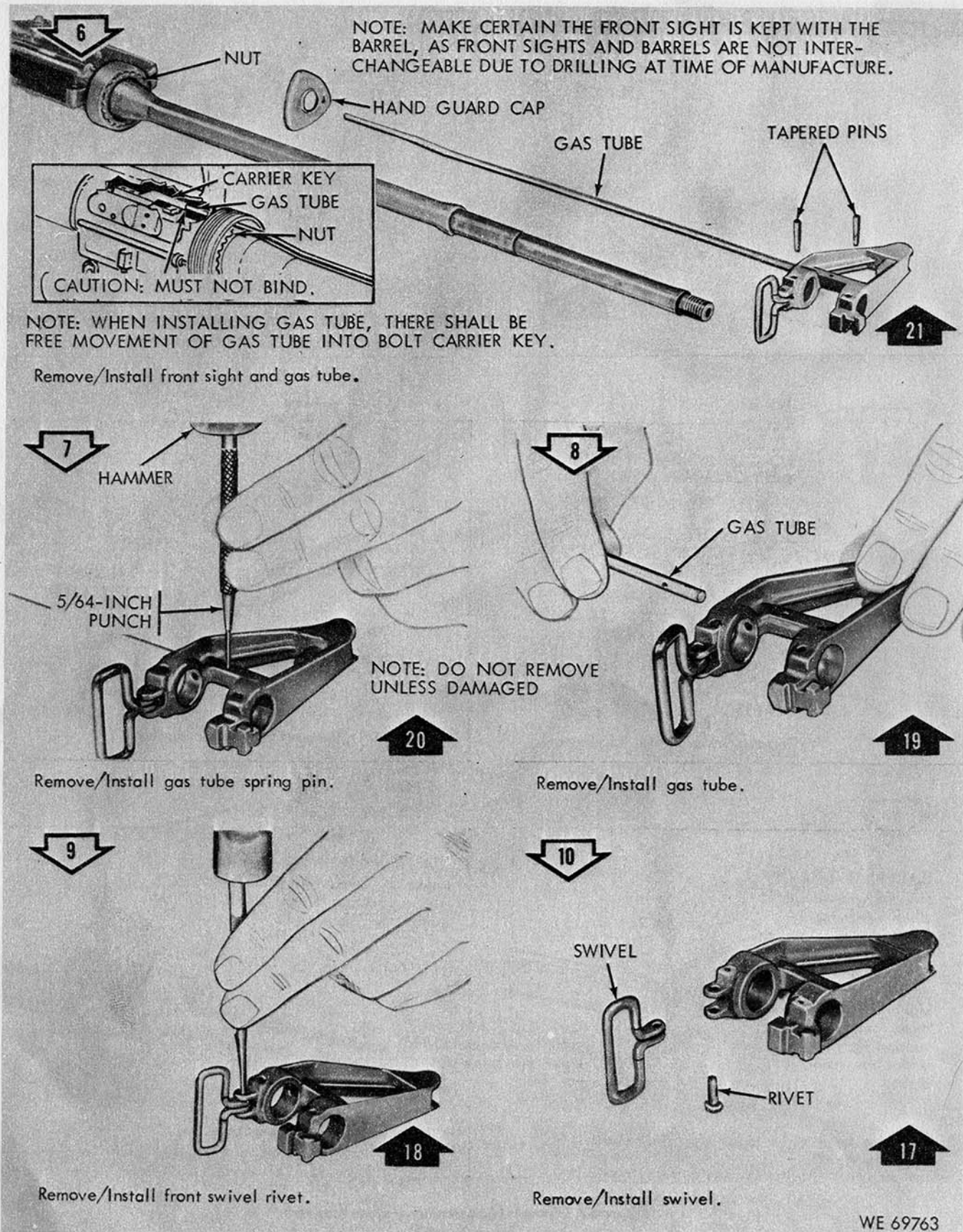
Figure 3-2. Disassembly/assembly of upper receiver group. (2 of 6)
