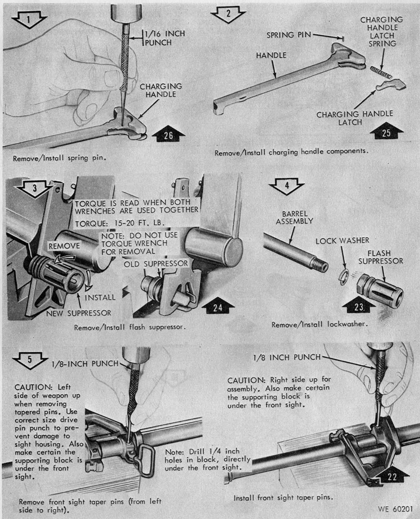
Figure 3-2. Disassembly/assembly of upper receiver group (1 of 6)
