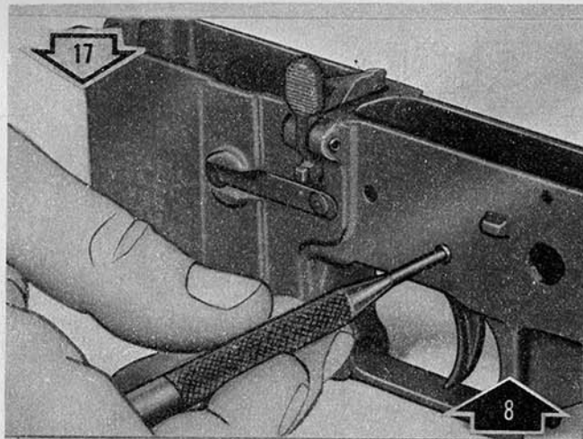
Remove/Install trigger pin.
