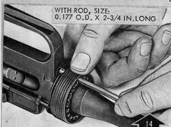
Remove/Install front sight post
