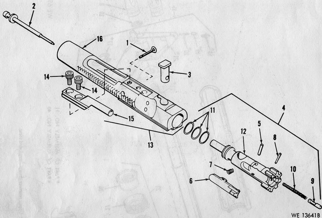
Figure B-3. Bolt carrier group—exploded view.
