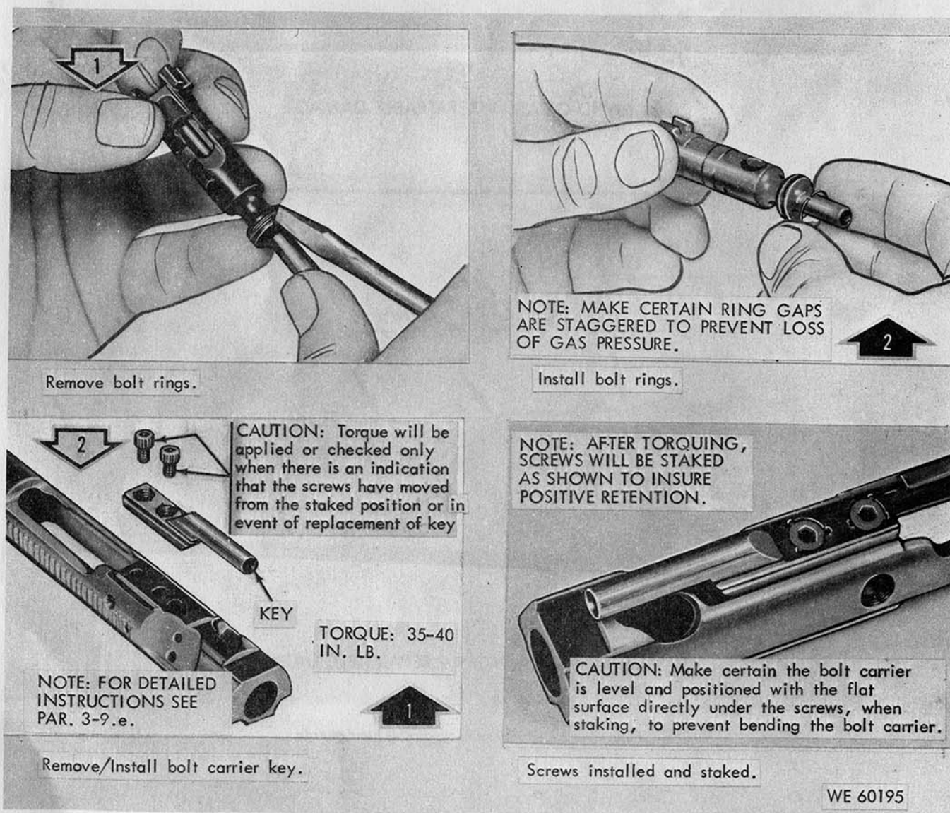
Figure 3-5. Disassembly/assembly of bolt carrier group.
