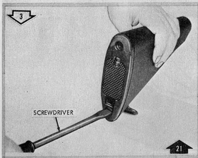
Remove/Install machine screw
