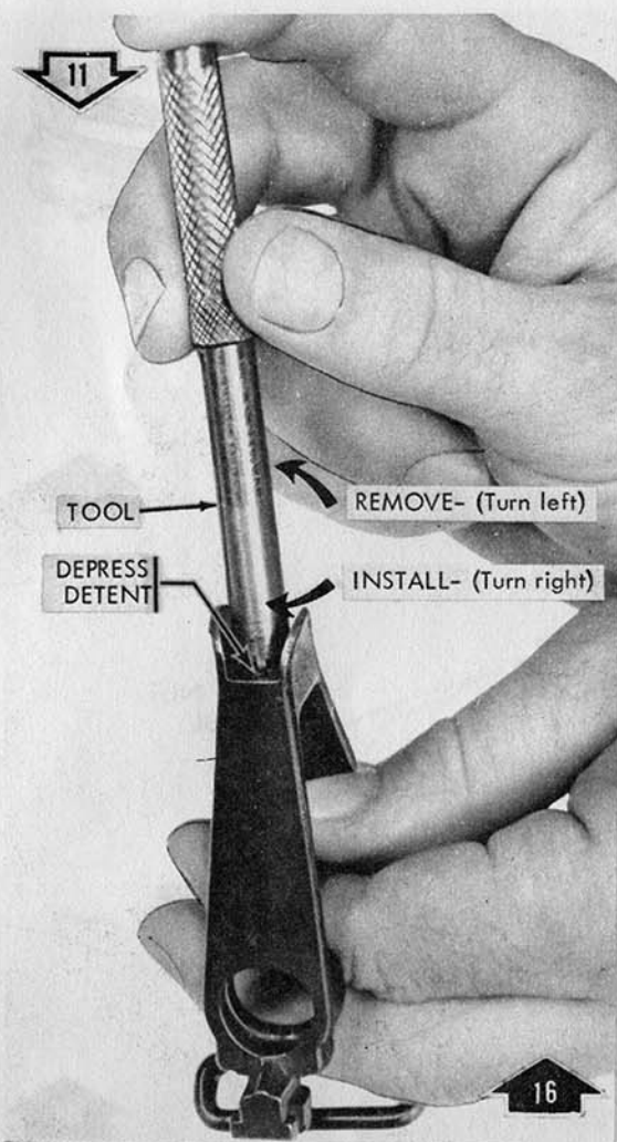
Remove/Install front sight post
