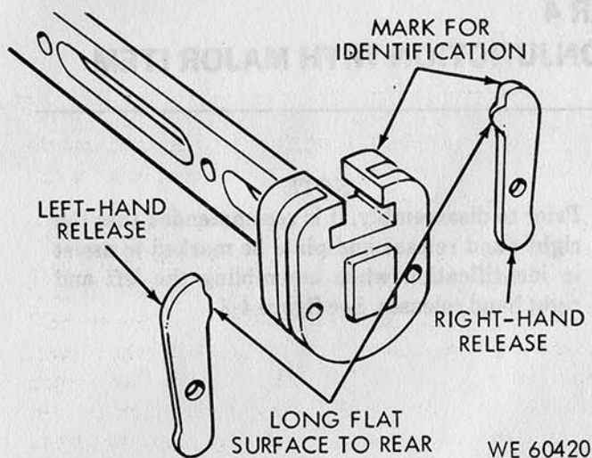
Figure 4-2. Bayonet-Knife—marking and identification of releases.
