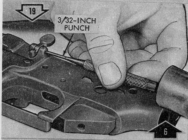
Remove/Install bolt catch spring pin.
