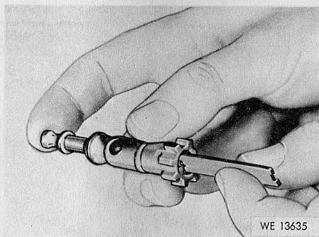
Figure 3-15. Check bolt with firing pin protrusion gage.
