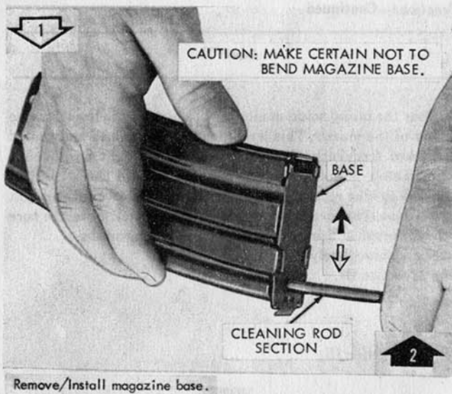
Figure 3-1. Disassembly/assembly of magazine assembly.
