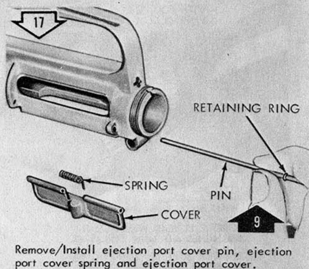
Figure 3-2. Disassembly/assembly of upper receiver group. (4 of 6)
