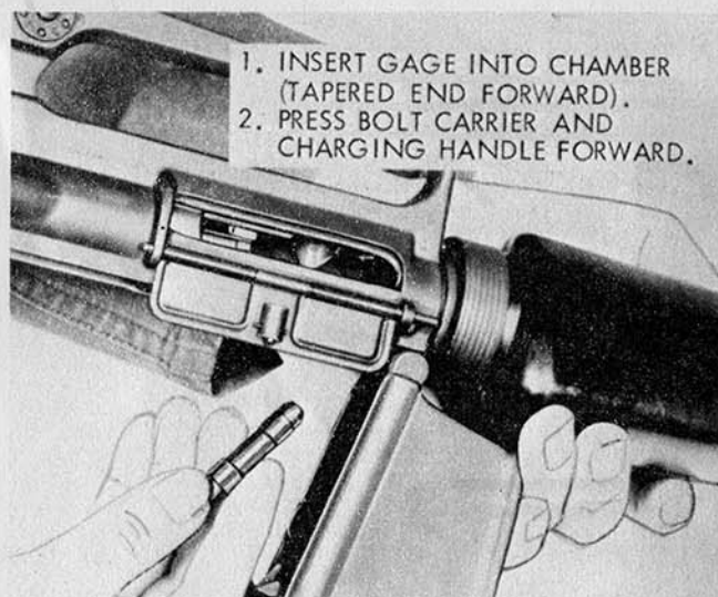
1. Inserting headspace gage.
