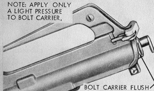
3. Incorrect headspace.
