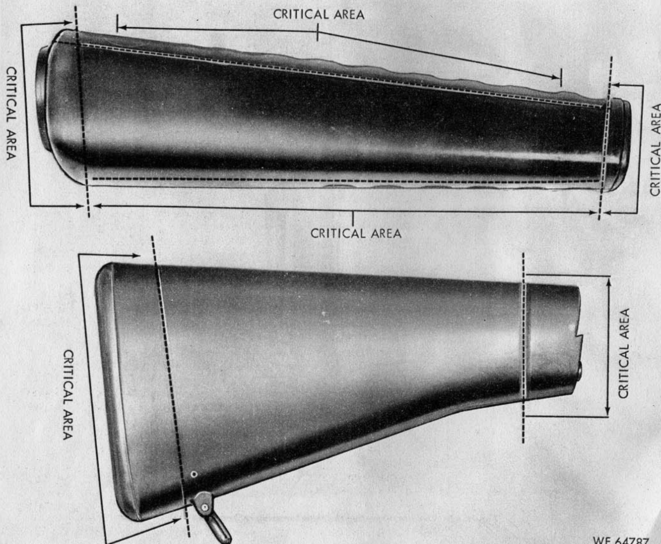
Figure 3-11. Critical areas of stock assembly and hand guard.
