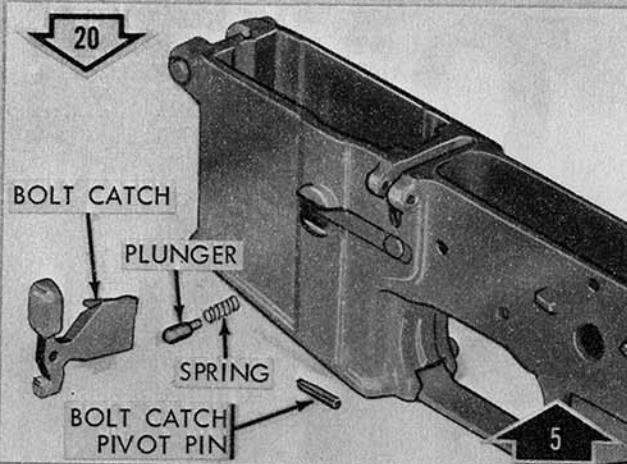
Remove/Install bolt catch, bolt catch plunger, and bolt catch spring.
