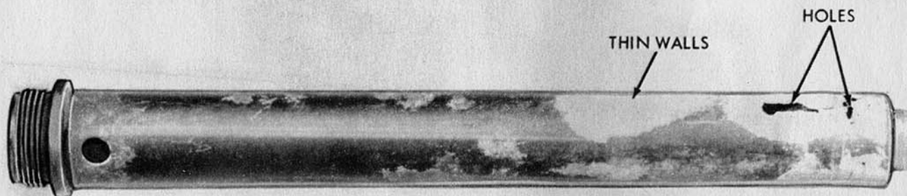
C - HOLES AND THIN WALLS - NON-REPAIRABLE
