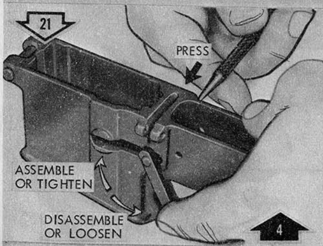
Remove/Install magazine catch.
