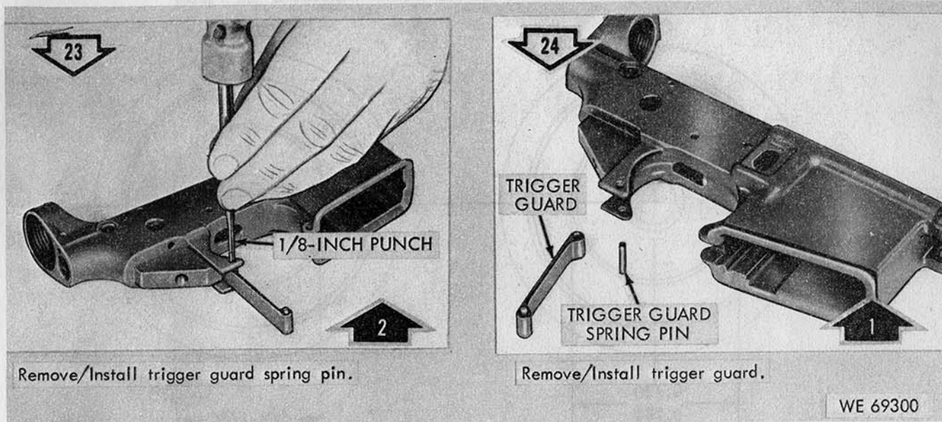
Figure 3-6. Disassembly/assembly of lower receiver group. (5 of 5)
