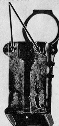
C - CORRODED LOBES - WEAKENING PIVOT PIN AREA NON-REPAIRABLE
