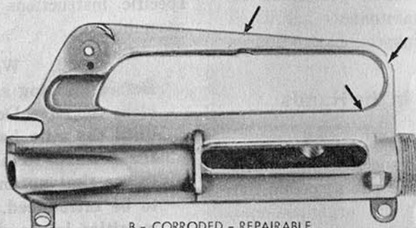
B - CORRODED - REPAIRABLE
