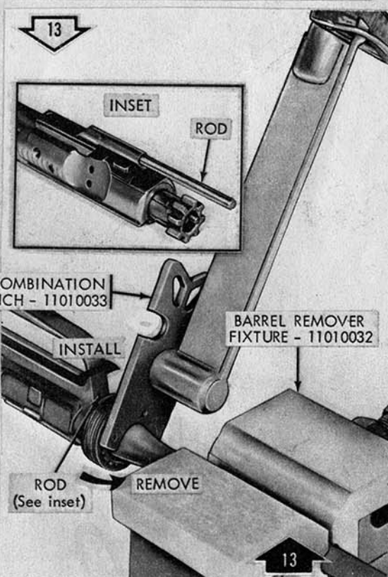
Remove/Install barrel nut assembly.
