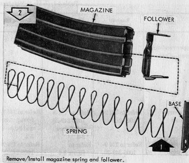
Figure 3-1. Disassembly/assembly of magazine assembly.
