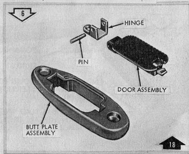
Remove/Install pivot latch pin and hinge.
