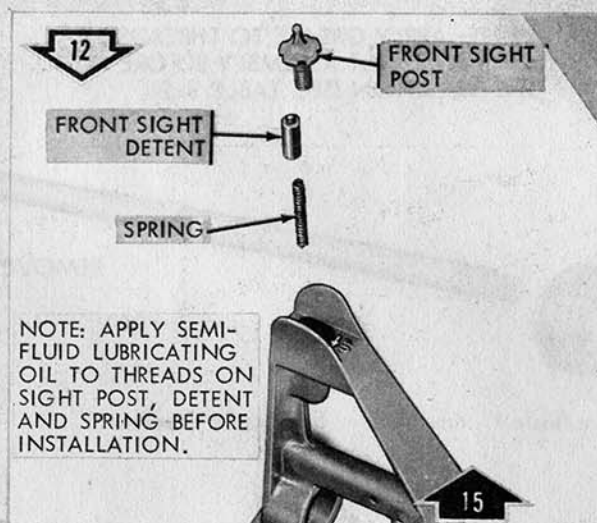
Remove/Install front sight detent and front sight spring.
