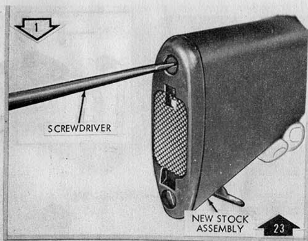
Remove/Install butt cap screw
