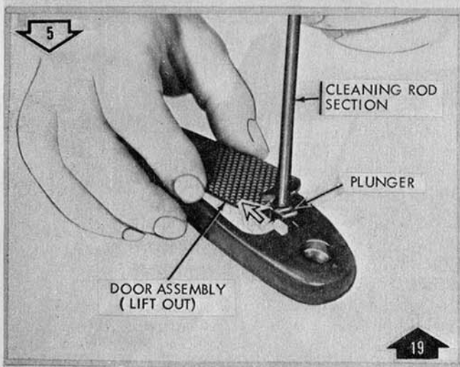
Unlock/Lock plunger and Remove/Install door assembly
