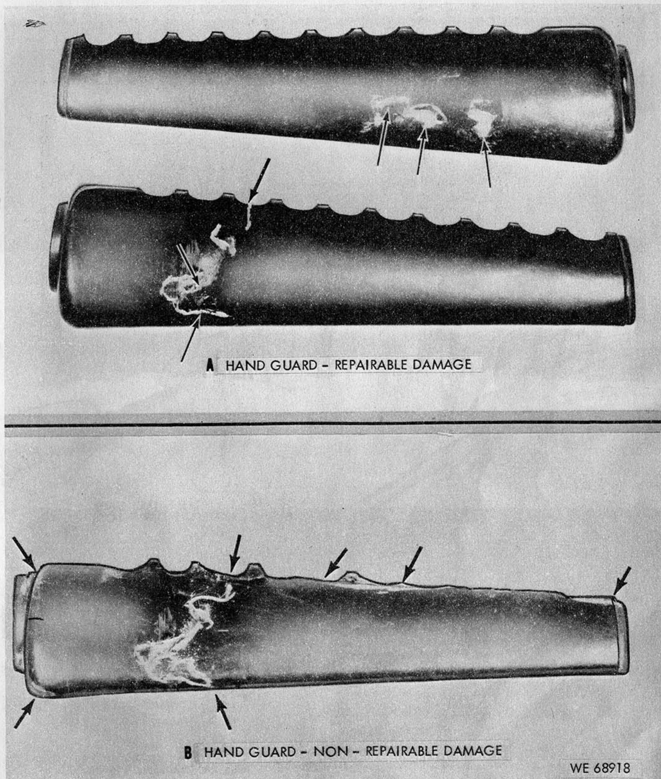
Figure 3-3. Repairable/non-repairable hand guards.
