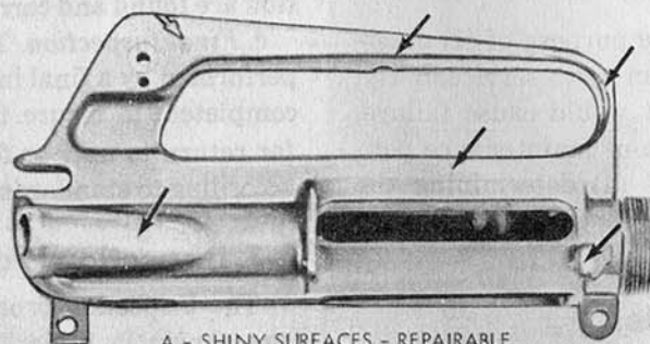
A - SHINY SURFACES - REPAIRABLE
