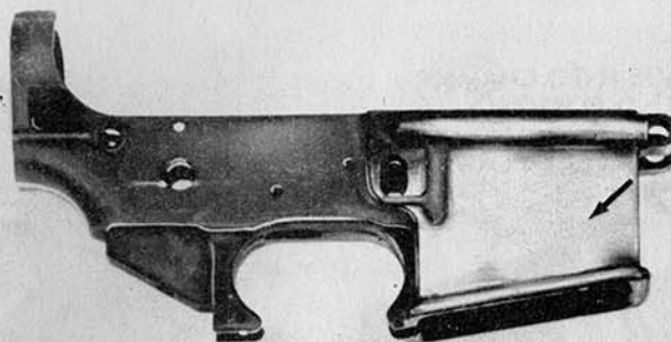
A - SHINY SURFACES - REPAIRABLE
