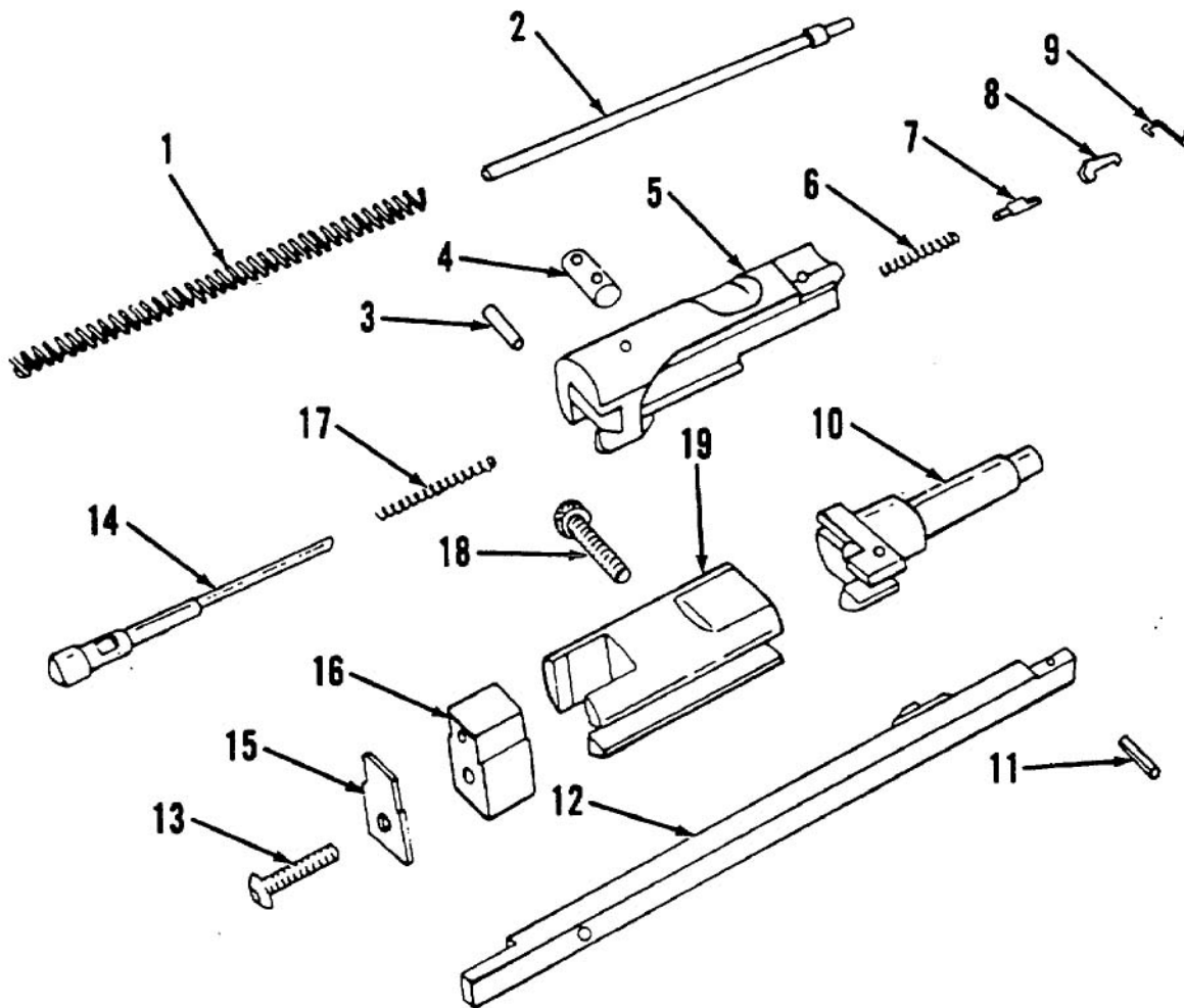
Figure D-2. Bolt adapter assembly 12003080
