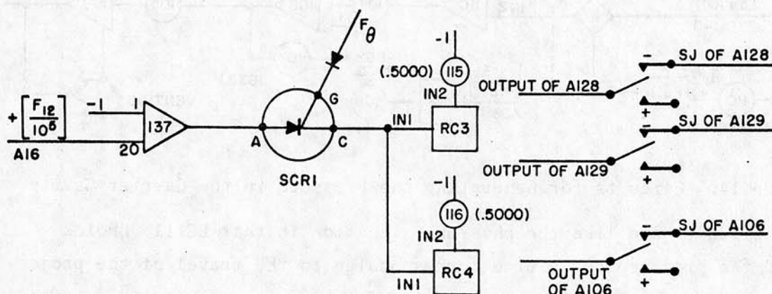
Figure 15. Control Circuits
