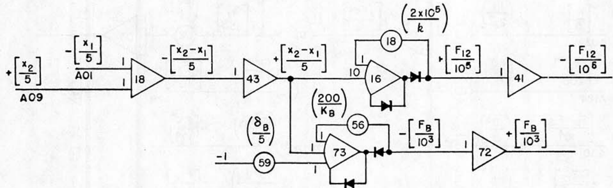
Figure 26. Circuits for Generating F_{12} and F_B
