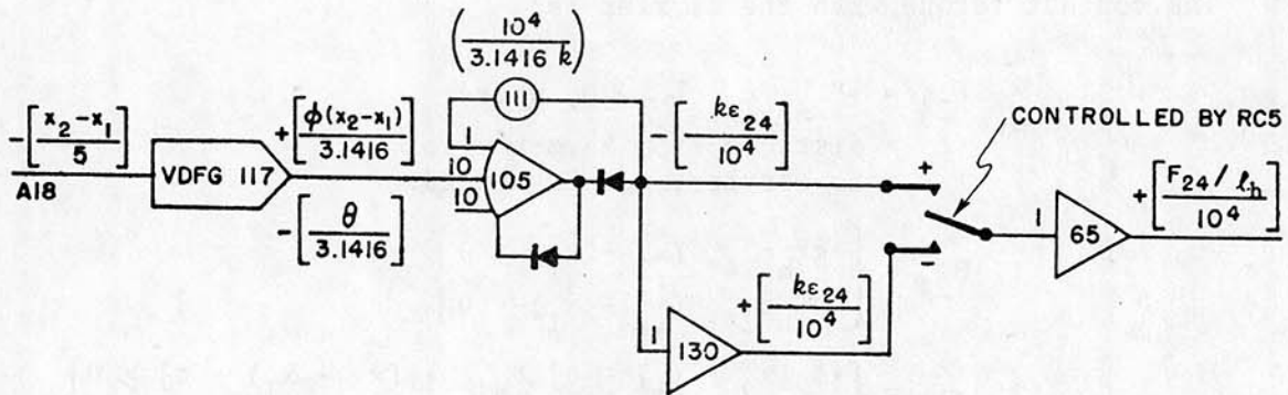
Figure 32. Circuits for Generating the Hammer-Carrier Force
