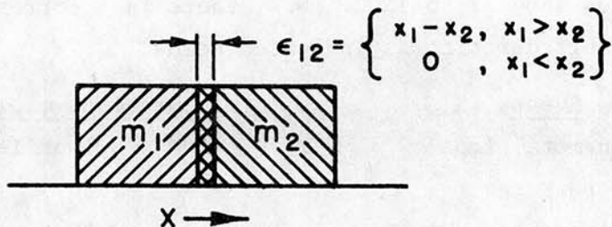
Figure 4. Impact From the Left
