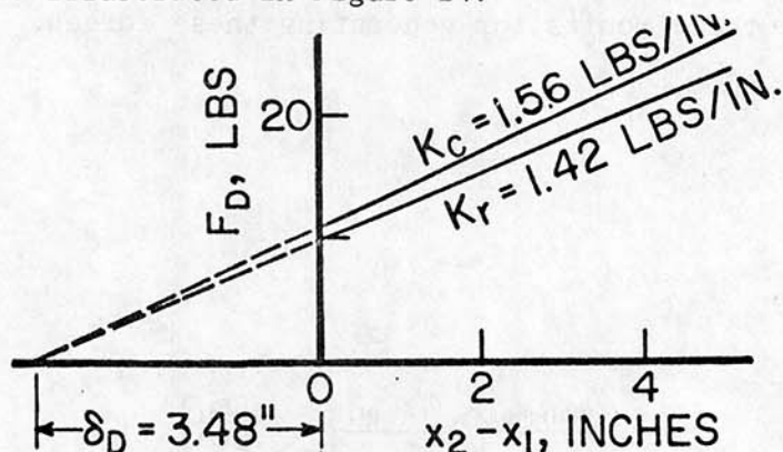
Figure 24. Driving Spring Force
