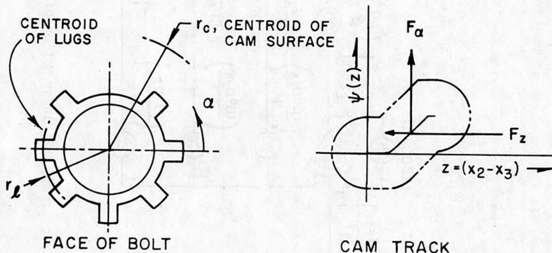
Figure 19. Diagram of Bolt Forces
