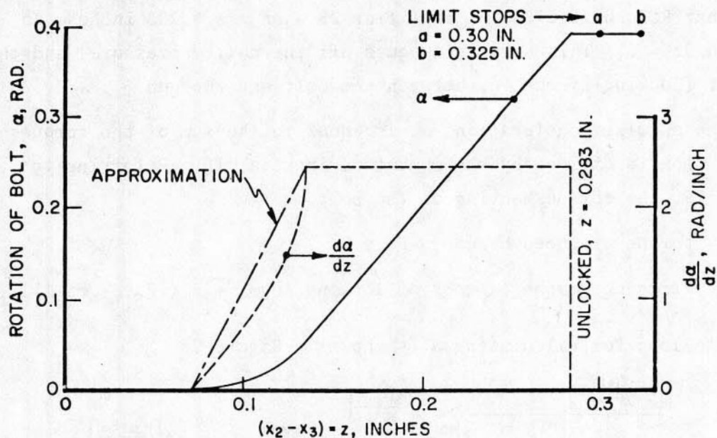
Figure 20. The Cam Track and Its Derivative
