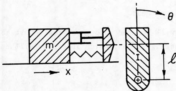
Figure 11. Combined Linear and Angular Impact
