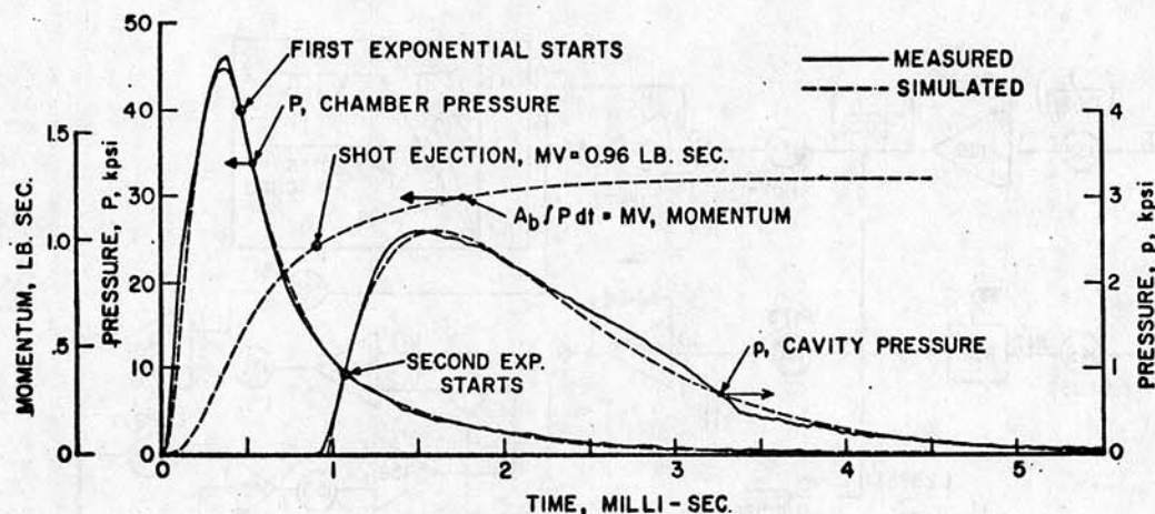
Figure 13. Pressure-Time Curves
