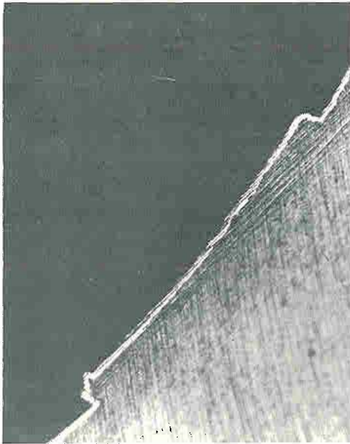
FIGURE 12 TYPICAL LAND PROFILE M16A1 RIFLE BARREL PROCESS "B" 100X
