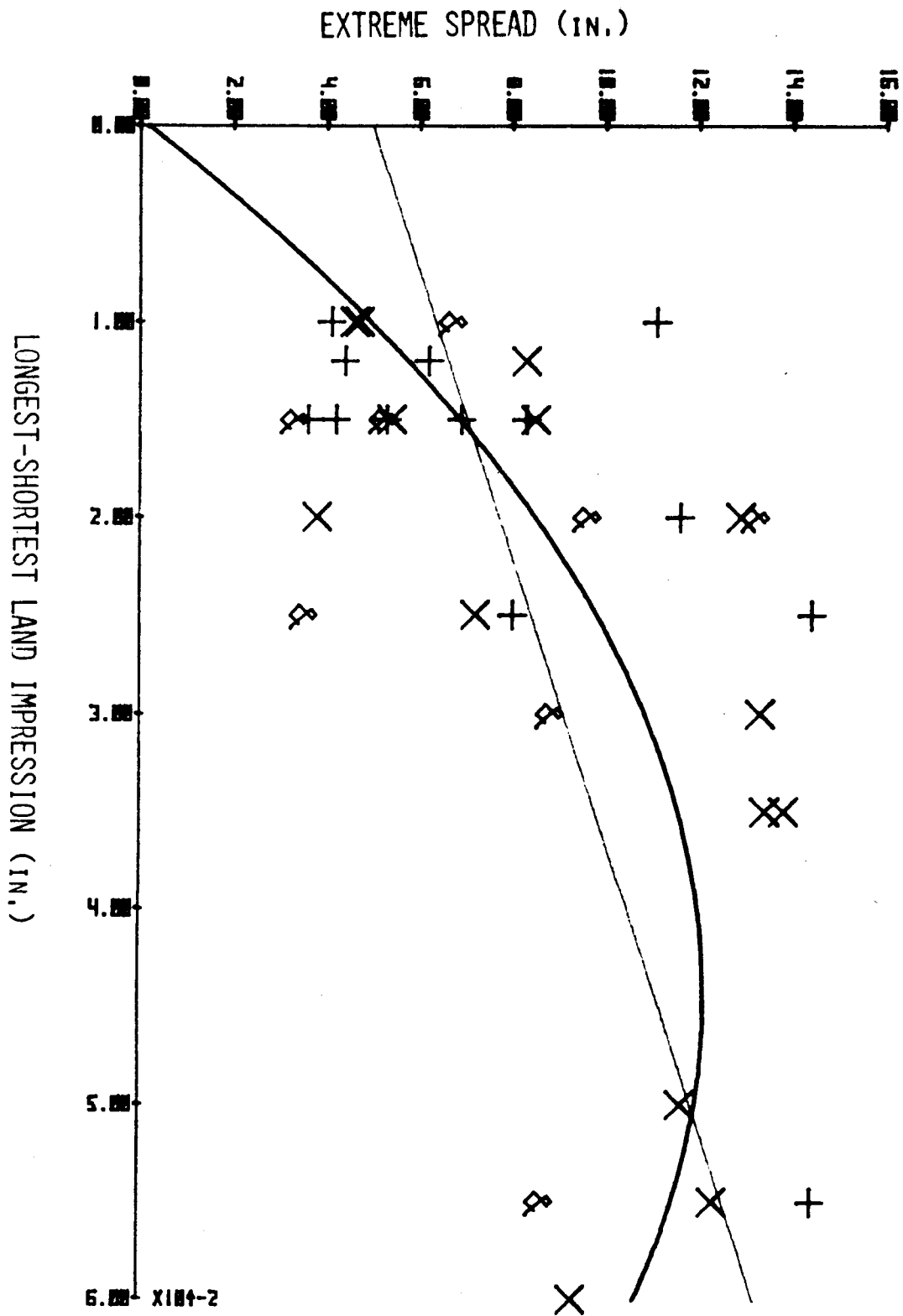
GRAPH 15 ALL RATES, PROCESS A, BALL AMMO
