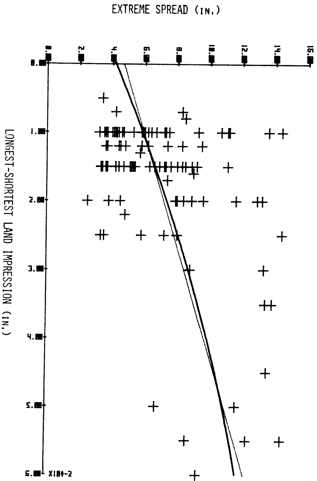
GRAPH 13 ALL RATES, ALL PROCESSES, BALL AMMO
