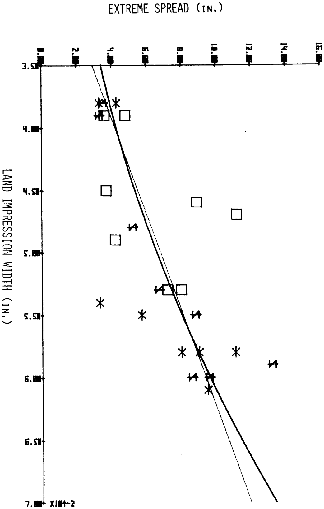
GRAPH 19 60 RDS PER MIN, ALL PROCESSES, BALL AMMO
