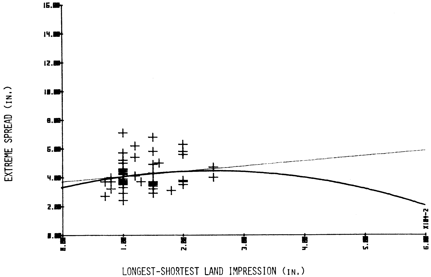
GRAPH 14 ALL RATES, ALL PROCESSES, TRACER AMMO
