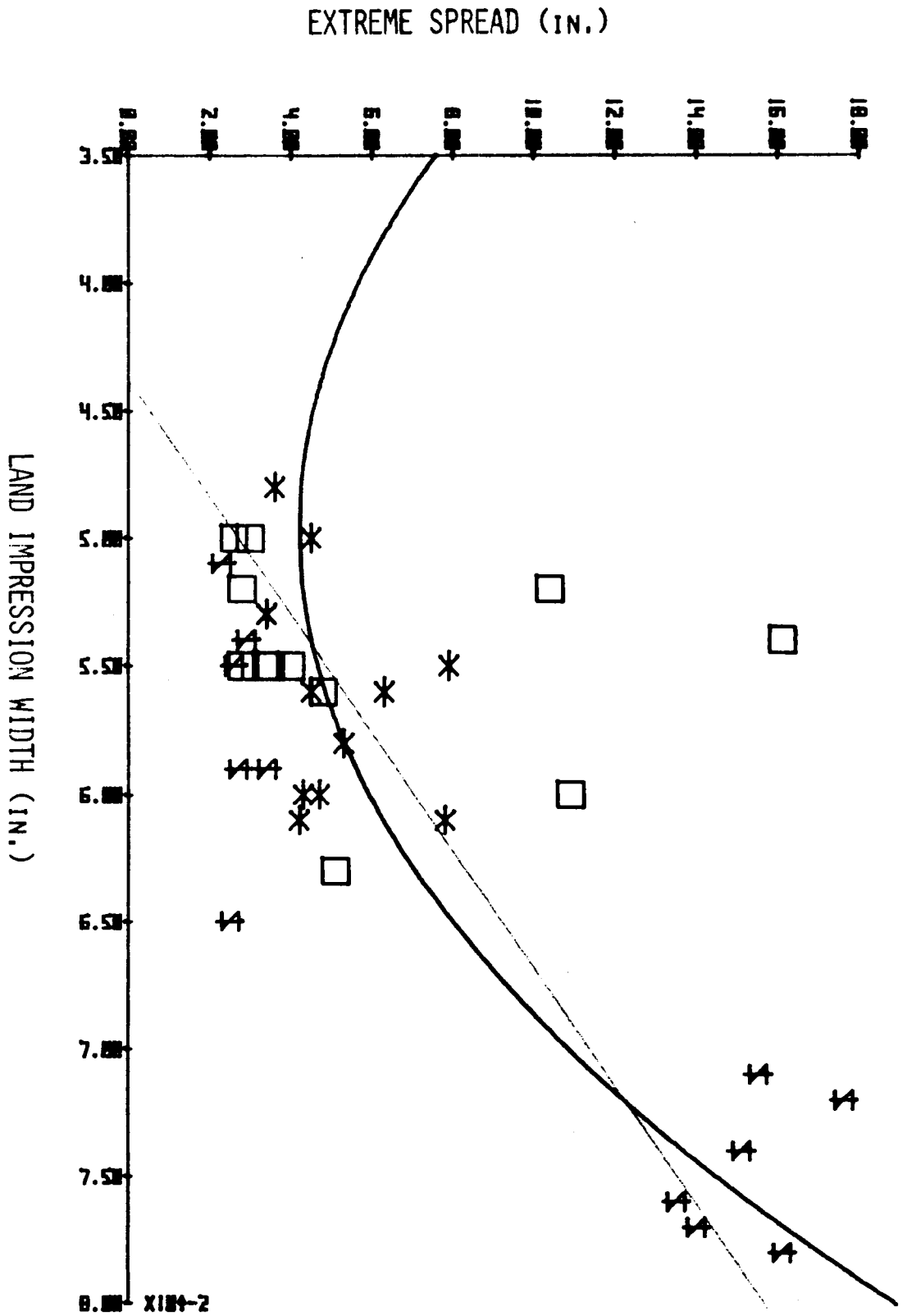
GRAPH 1 29 RDS PER MIN, ALL PROCESSES, BALL AMMO; TEST 1
