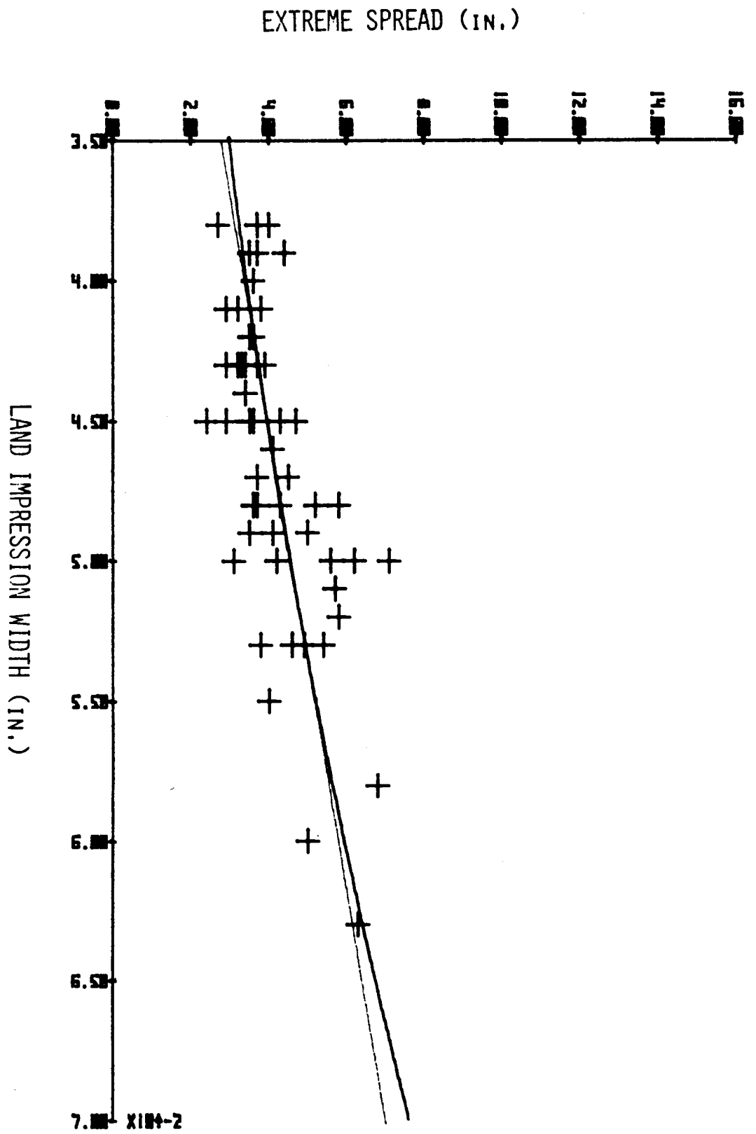
GRAPH 5 ALL RATES, ALL PROCESSES, TRACER AMMO
