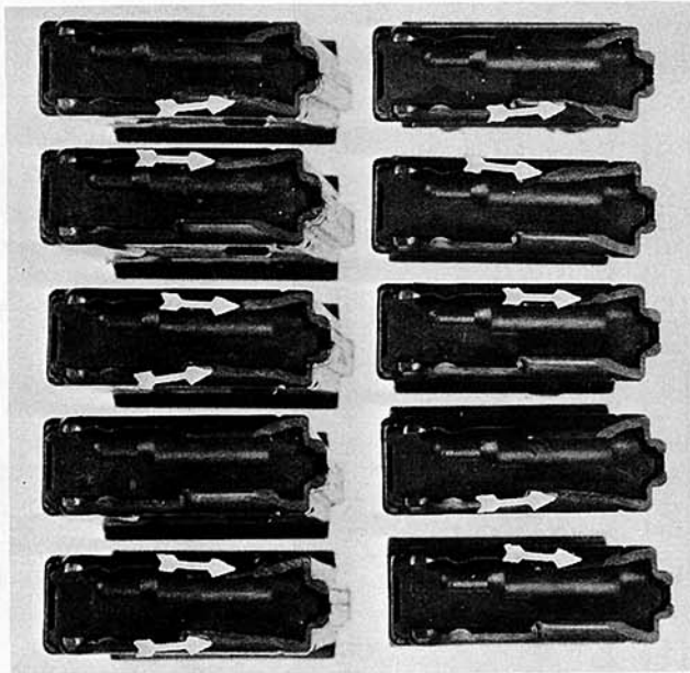
Figure 2.3-1: Material Damage to Third EDT (Type 1B) Magazines Caused by Drop Test at -65^{\circ}\text{F} onto Concrete Surface. Note Feed-Lip Breakage.
