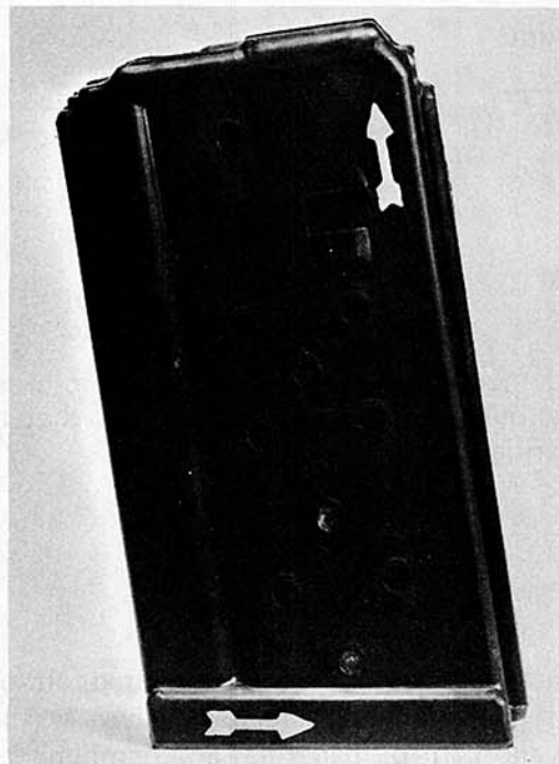
Figure 2.2-2: Second Engineer Design Test (EDT) Magazine (Type 1A) Showing Left Side View. Note the Absence of Vertical Groove at Top Rear of Magazine Which Facilitates Attachment of Magazine Filler, and the Difference of the Base Configuration to That of Figure 2.2-4.
