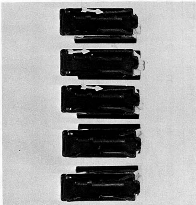
Figure 2.3-2: Material Damage to Third EDT (Type 1B) Magazines Caused by Drop Test at -65^{\circ}\text{F} onto 3/8-Inch Plywood. Note Damage Similar to Figure 2.3-1.
