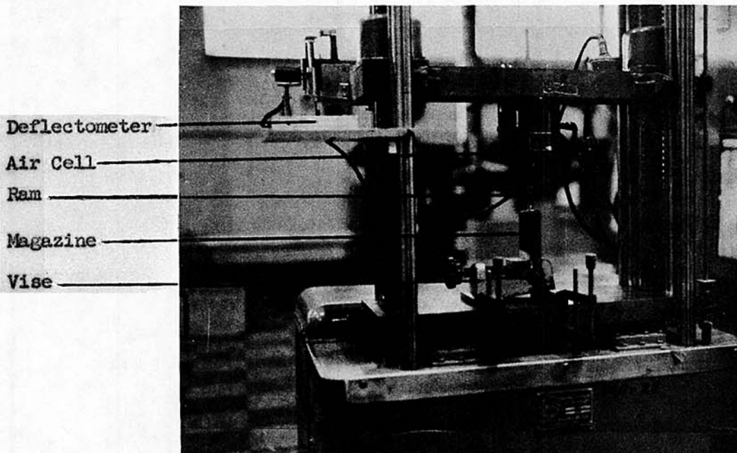
Figure I-1: Setup for Load Deflection Testing of Magazines for 5.56-MM Ammunition for M16 Rifles.
