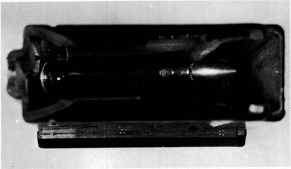
Figure 2.8-1: Top View of Cartridge (Round 20) and Follower Jammed in Test Magazine. Note the Granules of Sand Lodged between Side (Left Rear) of Cartridge Case and Magazine.
