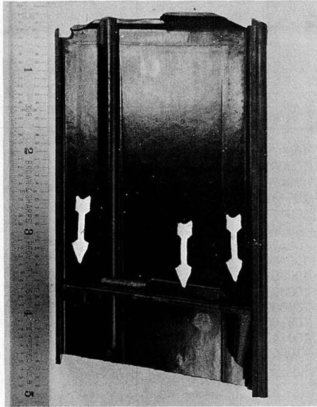
Figure 2.2-9: Cutaway View (Left Side Removed) of the Interior Configuration of the Test Magazine with Redesigned Follower Positioned toward the Bottom of the Magazine. The Three Arrows Indicate the Contact Surfaces of the Follower and Magazine Body Which Causes Seizure between These Components and Prevents Upward Movement of the Ammunition Stack during Firing in Adverse Conditions.
