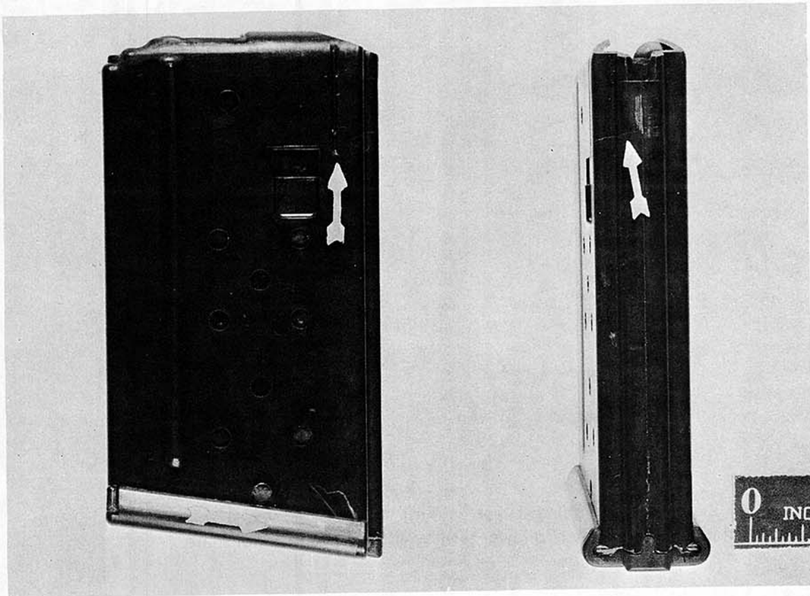
Figure 2.2-4: LEFT: Side View Showing Design Changes of Third EDT Magazine (Type 1B). RIGHT: Rear View of Same Magazine Displaying Die Crack Mark.
