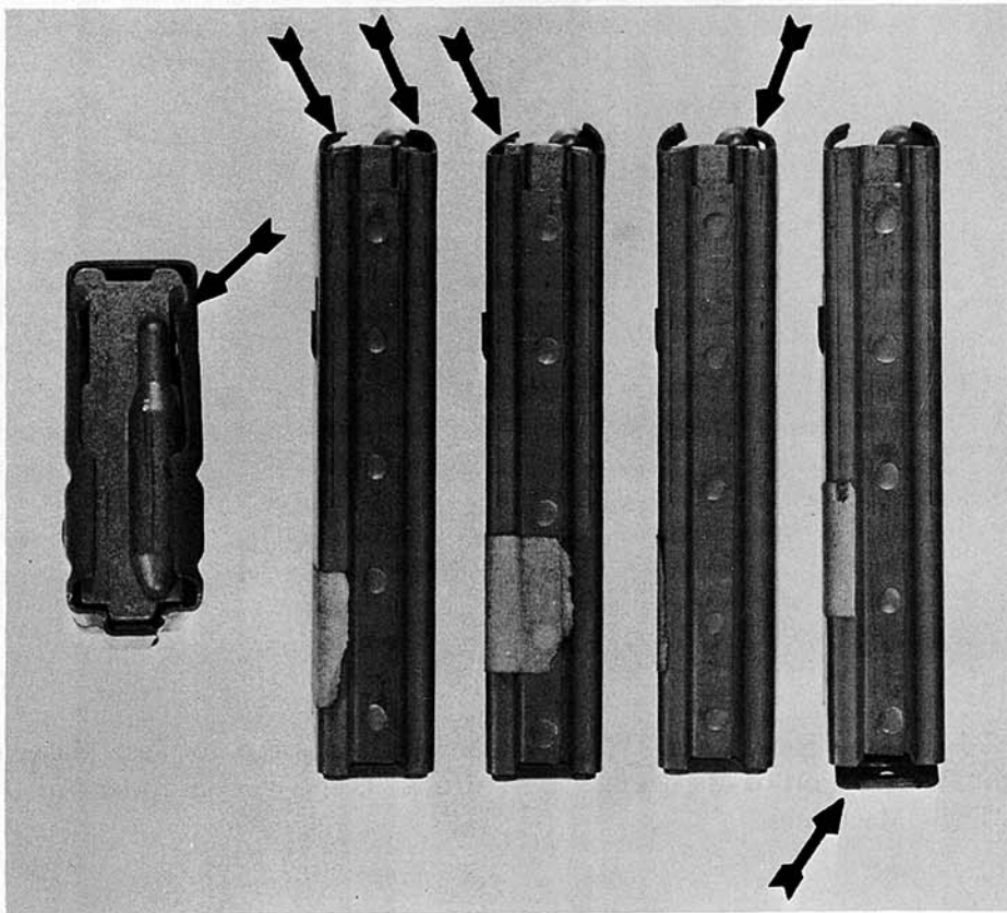
Figure 2.4-1: Five-Foot Drop Test Damage to Control Magazines at +155°F. LEFT to RIGHT: Top Forward Portion of Right Feed-Lip Bent Inward; Three Magazines with Deformed Rear Portion of Feed-Lip; and One Magazine with Floor Plate Damage. Similar Results Occurred at -65 F.
