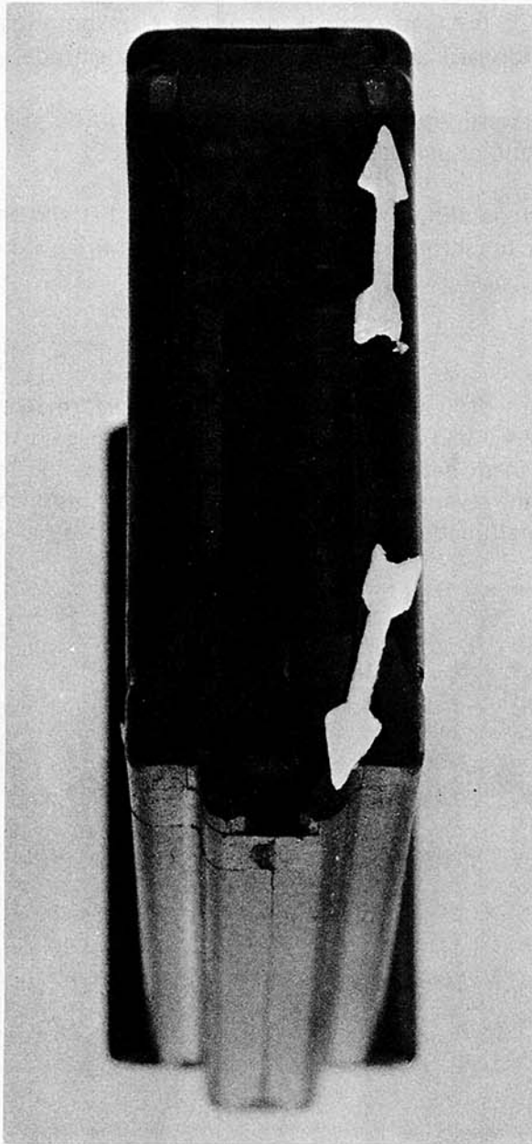
Figure 2.4-2: Five-Foot Drop Test. Representative Damage to Test Magazines at +155°F. Slight Deformation of Magazine Body (Arrows) Is the Normal Extent of Damage Occurring on These Magazines.
