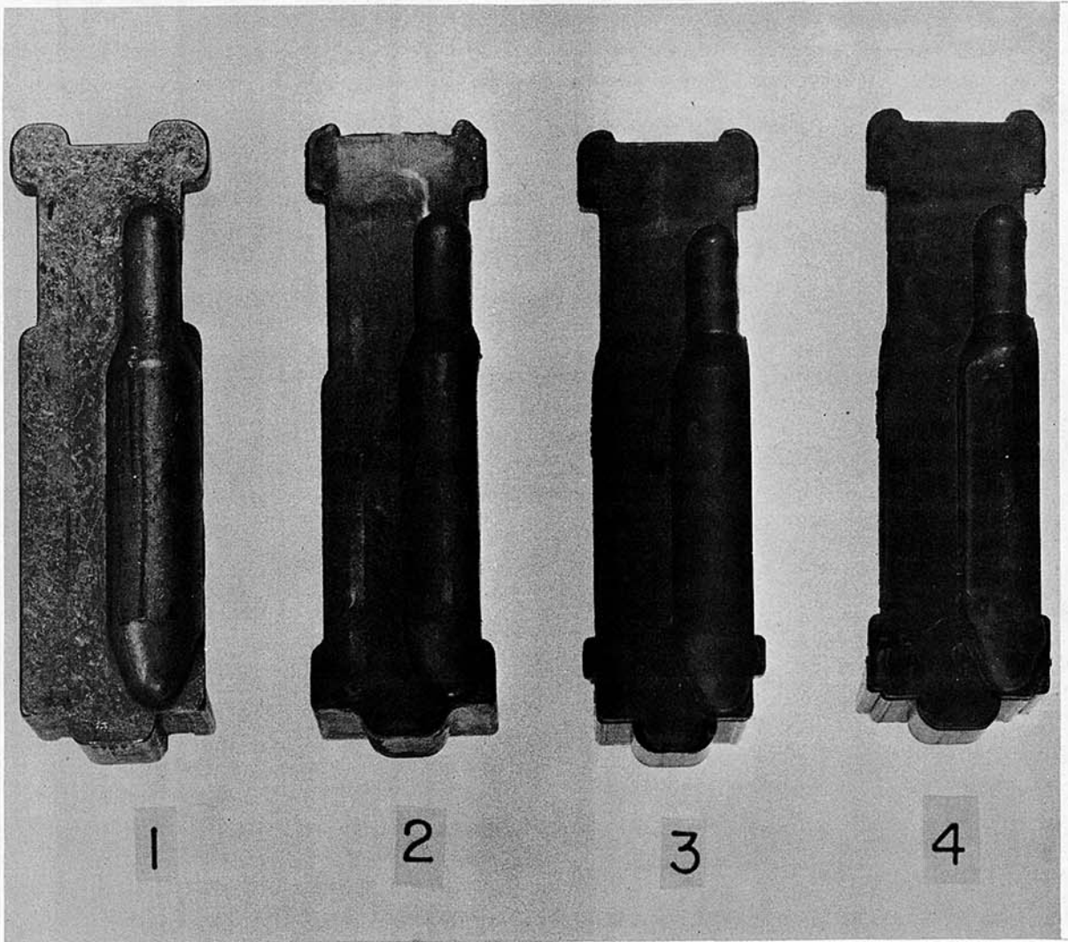
Figure 2.2-6: Comparison of Magazine Follower Designs: 1. Control Magazine. 2. Second EDT (Type 1A) Magazine. 3. Third EDT (Type 1B) First Design. 4. Third EDT (Type 1B) Second Design. (Nos. 2, 3, and 4 are Test Magazines.)
