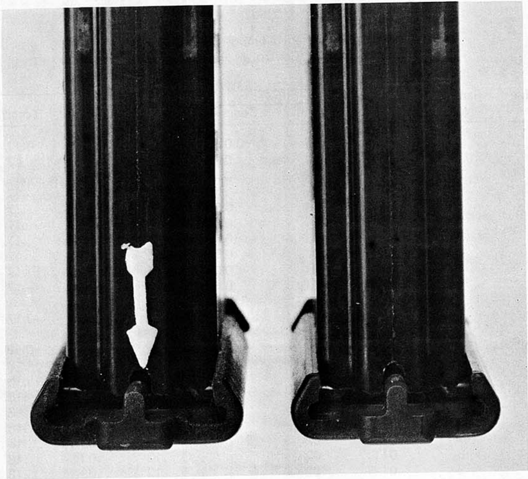
Figure 2.2-8: Rear View of the Test Magazine No. 168 Showing Irregularities of Floor Plate Latch Detent (LEFT) and a Normal Magazine (RIGHT) for Comparison.
