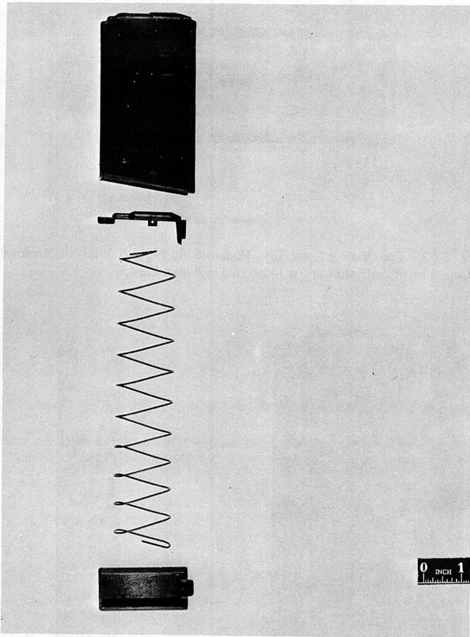
Figure 2.2-5: Disassembled View of Test Magazine (Type 1B) Showing (TOP to BOTTOM) the Magazine Body, Follower, Follower Spring, and Floor Plate.
