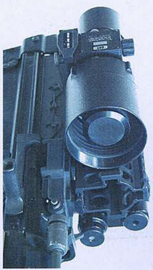
Lower profile KnightSight™ Mounting.
