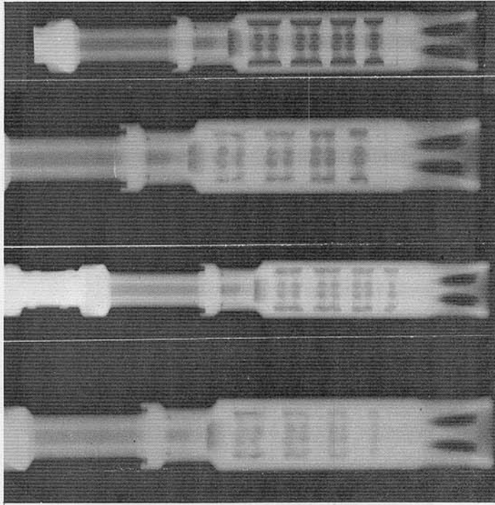
Figure 2.2-10: Flash Suppressor of XM177E2, No. 904546 before Firing and after Firing 1000, 5135, and 6515 Rounds (TOP to BOTTOM).
