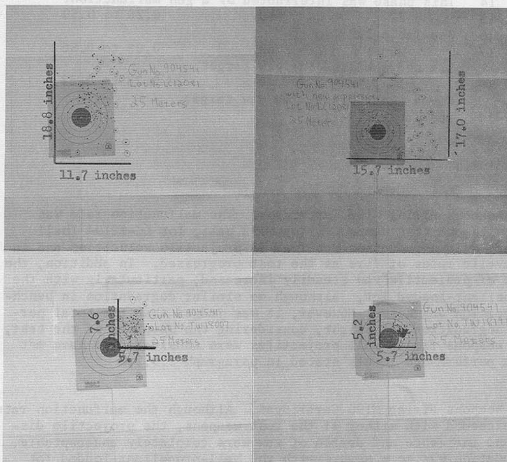
Figure 2.9-1: Typical 120-Round, 25-Meter Targets Fired with Gun No. 904541 and Various Lots of Ammunition. Circled Projectile Impacts Indicate Severe Yaw. Rate of Fire, 15 Rds/Min.
