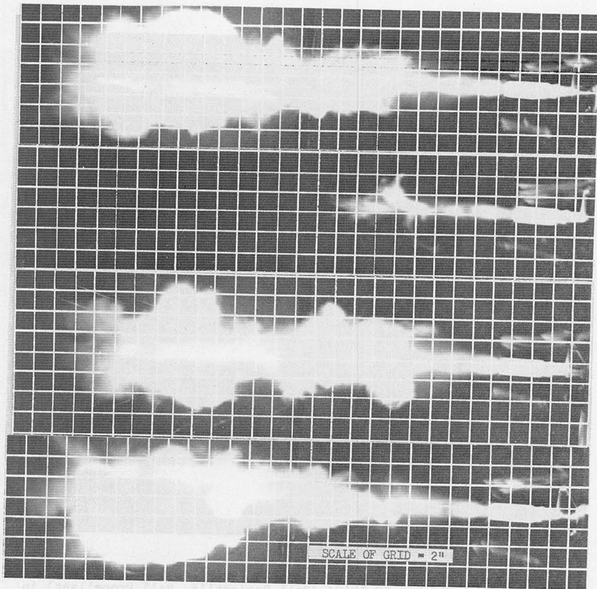
Figure I-6: Cumulative Muzzle Flash Photographs Obtained while Firing 30 Rounds of Lot LC-12194 (Ball Projectile, Ball Propellant) in a Used Condition (Fired More than 5100 Rounds) XM177E2 Submachine Gun. TOP TO BOTTOM: Fired Semiautomatically from Cold Barrel; Semiautomatically from Preheated Barrel (Heated First by Firing 60 Rounds); Automatically from Cold Barrel; Automatically from Preheated Barrel.
