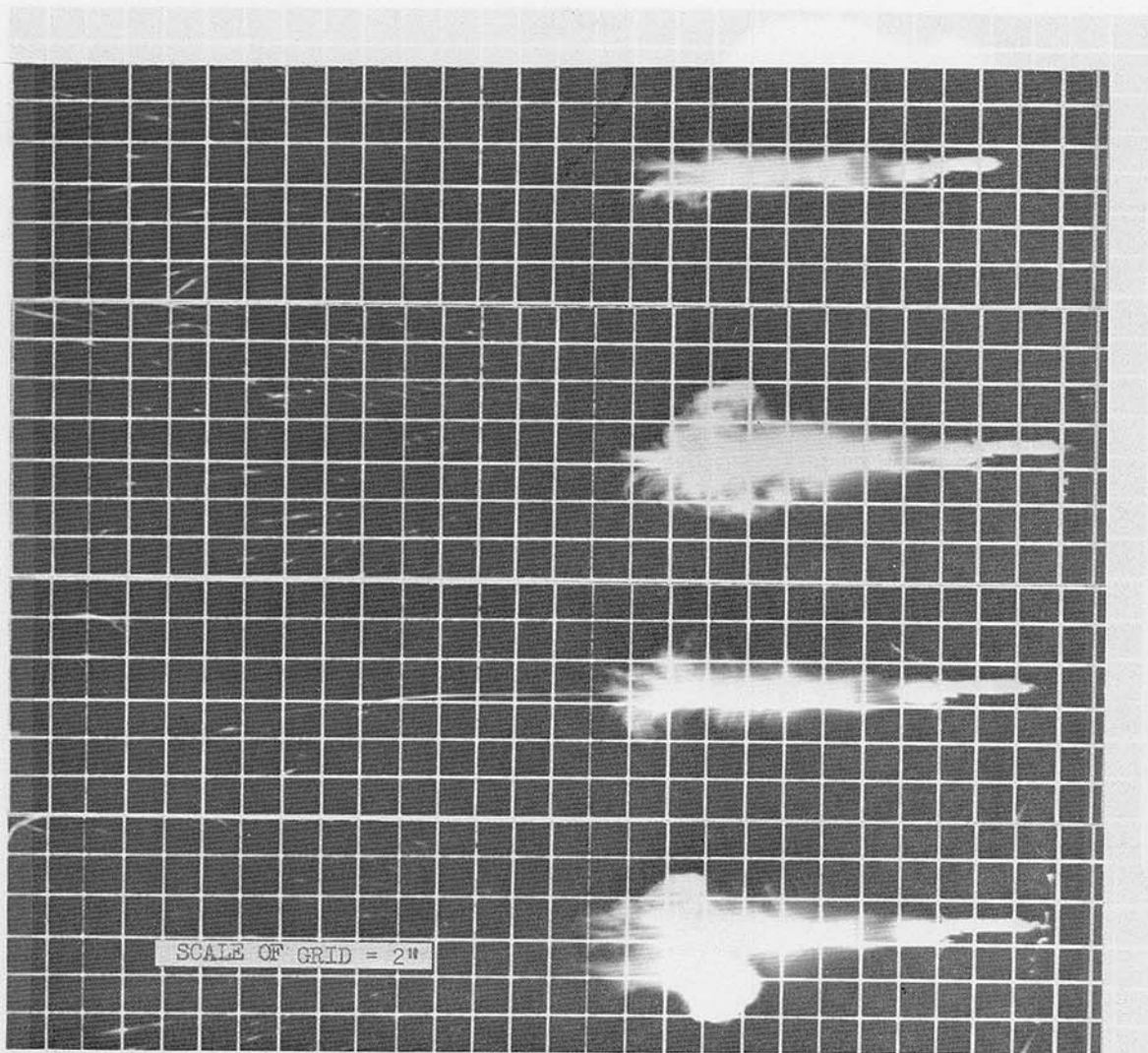
Figure I-5: Cumulative Muzzle Flash Photographs Obtained while Firing 30 Rounds of Lot LC-12194 (Ball Projectile, Ball Propellant) in a New Condition (Less than 300 Rounds) XM177E2 Submachine Gun. TOP TO BOTTOM: Fired Semiautomatically from Cold Barrel; Semiautomatically from Preheated Barrel (Heated First by Firing 60 Rounds); Automatically from Cold Barrel; Automatically from Preheated Barrel.
