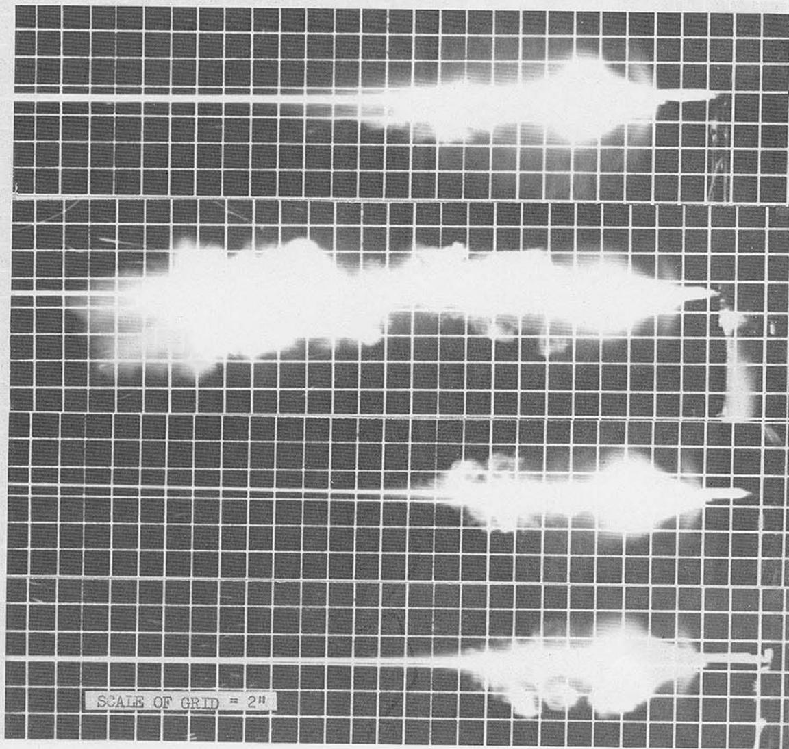
Figure I-1: Cumulative Muzzle Flash Photographs Obtained while Firing 30 Rounds of Lot LC-12081 (Tracer Projectile, Ball Propellant) in a New Condition (Less than 300 Rounds) XM177E2 Submachine Gun. TOP TO BOTTOM: Fired Semiautomatically from Cold Barrel; Semiautomatically from Preheated Barrel (Heated First by Firing 60 Rounds); Automatically from Cold Barrel; Automatically from Preheated Barrel.
