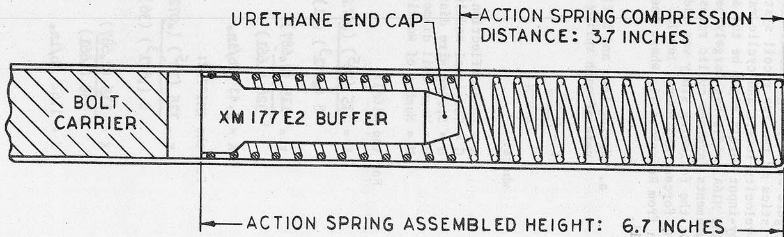
Figure 2.16-1: Engineering Sketch of the Buttstock Extension Tube, Buffer, and Action Spring for the M16A1 Rifle and XM177E2 Submachine Gun.
