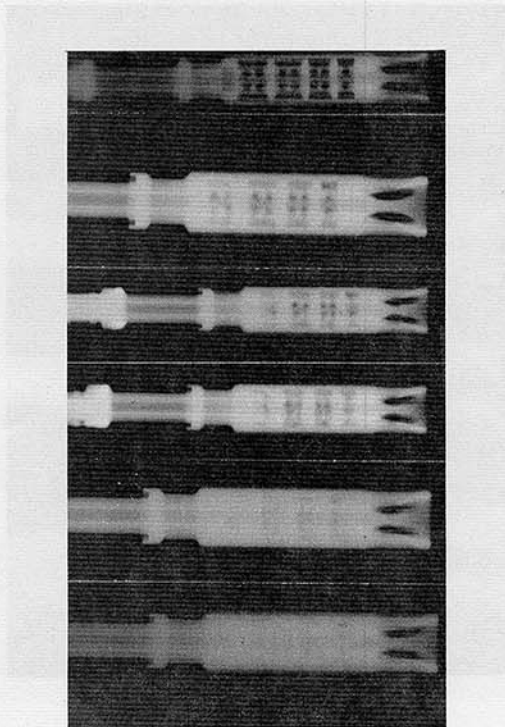
Figure 2.2-6: Flash Suppressor of XM177E1, No. 902279 before Firing and after Firing 1000, 2500, 4000, and 5500 Rounds (TOP to BOTTOM).
