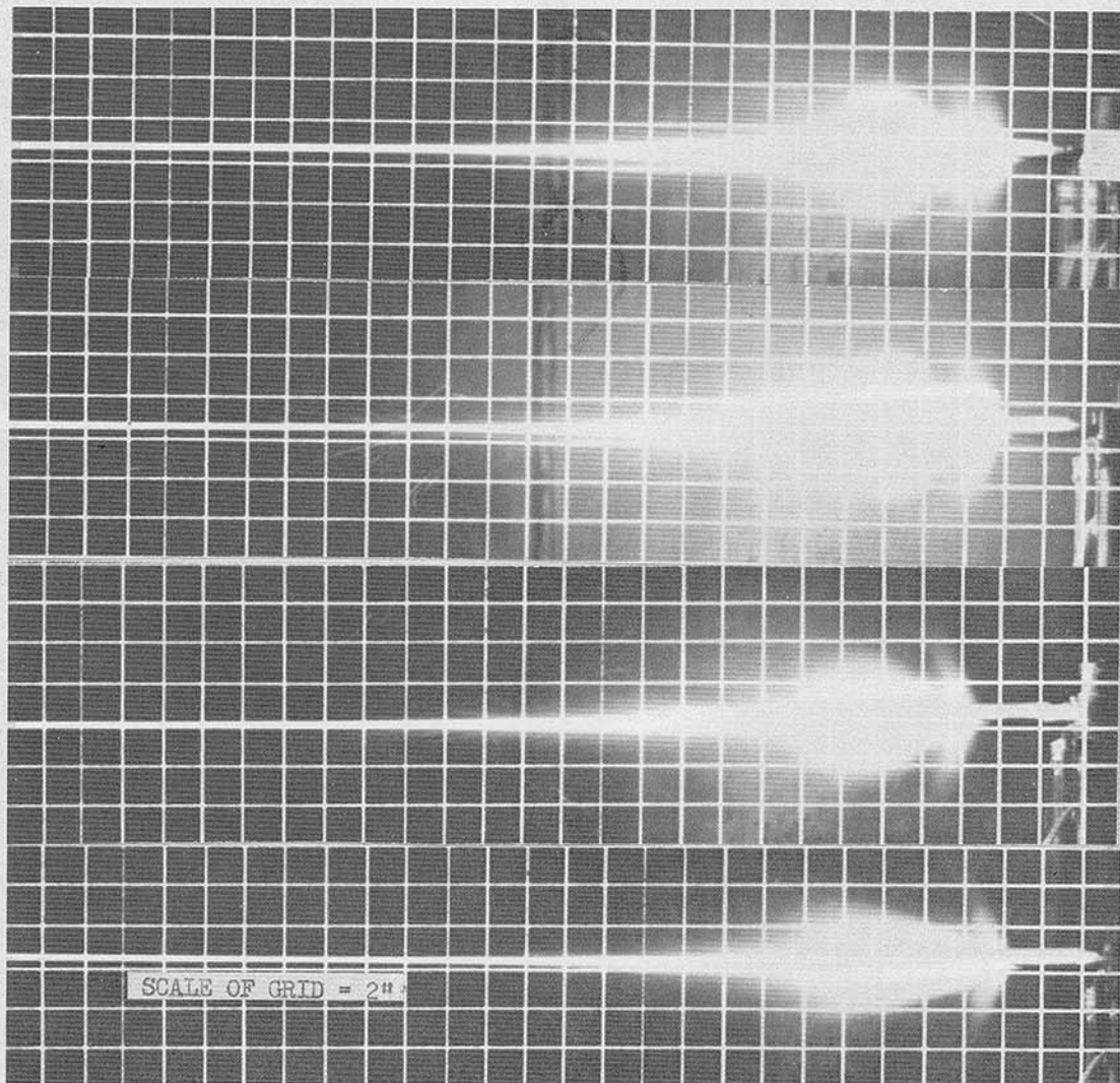
Figure I-3: Cumulative Muzzle Flash Photographs Obtained while Firing 30 Rounds of Lot TW-18007 (Tracer Projectile, 8208M Propellant) in a New Condition (Less than 300 Rounds) XM177E2 Submachine Gun. TOP TO BOTTOM: Fired Semiautomatically from Cold Barrel; Semiautomatically from Preheated Barrel (Heated First by Firing 60 Rounds); Automatically from Cold Barrel; Automatically from Preheated Barrel.
