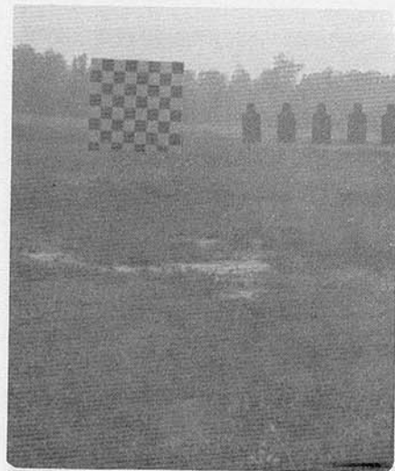
Figure I-11: Target Obscuration Effect of Smoke while Firing Automatically, Ten Rounds Each of Four Lots of Ammunition in XM177E2 Submachine Gun. UPPER LEFT: Lot LC-12081 (Tracer Projectile, Ball Propellant). UPPER RIGHT: Lot TW-18007 (Tracer Projectile, 8208M Propellant). LOWER LEFT: Lot LC-12194 (Ball Projectile, Ball Propellant). LOWER RIGHT: Lot TW-18191 (Ball Projectile, 8208M Propellant).
