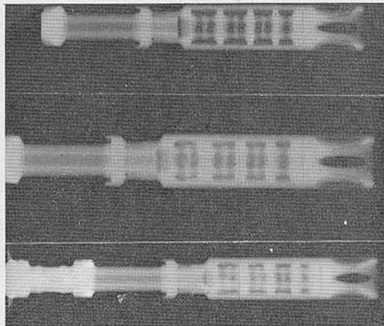
Figure 2.2-9: Flash Suppressor of XM177E2, No. 90454 before Firing and after Firing 1000 and 5167 Rounds (TOP to BOTTOM).
