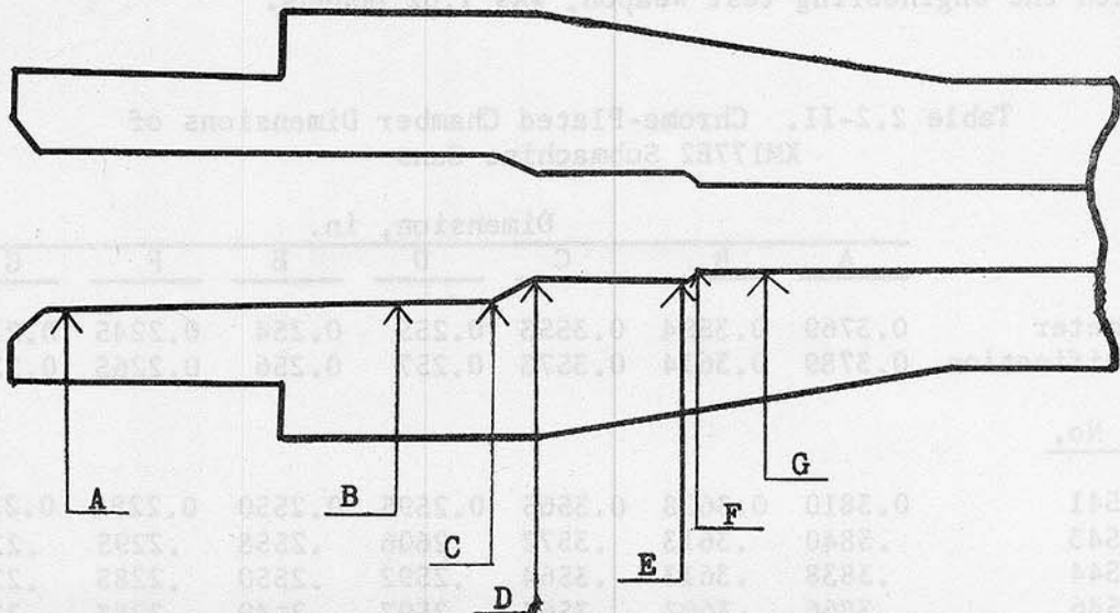
Figure 2.2-4: Sketch of Chamber for M16A1 Rifle and XM177E2 Submachine Gun. Letters Indicate Positions of Diameter Specifications as Shown on Standard Operation Instruction Sheet Used by the Manufacturer.
