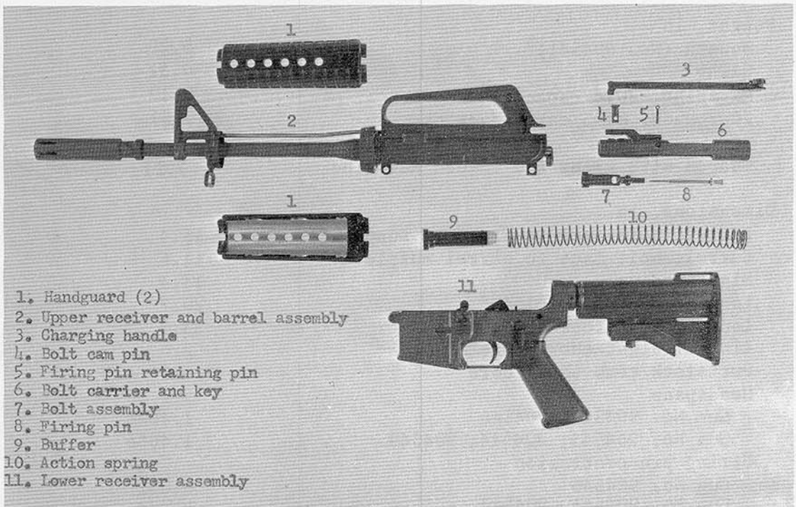
Figure 2.2-3: Field-Stripped XM177E2 Weapon.
