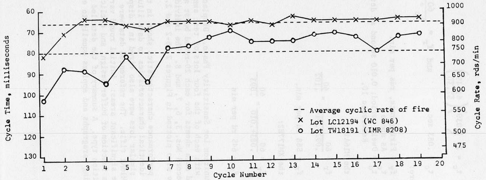
Figure 2.16-2: Cycle Times and Rates for Individual Rounds during Burst Fire with M193 (Ball Projectile) Ammunition.
