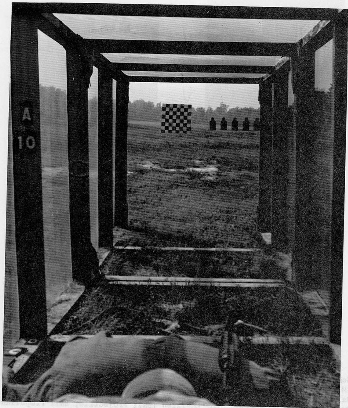
Figure I-9: Reference Photographs, Nonfiring, for Target Obscuration Test of XM177E2 and XM177E1 Submachine Guns. Checkerboard Target and E-Type Silhouettes Are at 50-Meter Range.
