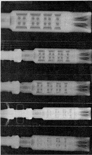
Figure 2.2-6: Flash Suppressor of XM177E1, No. 902279 before Firing and after Firing 1000, 2500, 4000, and 5500 Rounds (TOP to BOTTOM).
