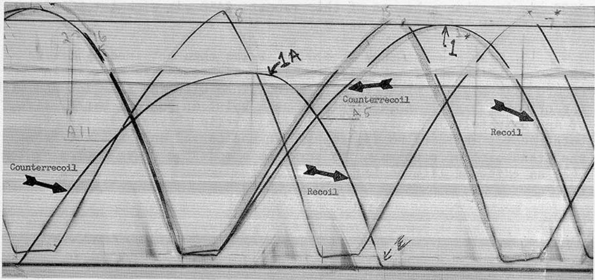
Figure 2.16-8: Displacement-Time Record During Burst Fire, Lot LC12081, Record No. 8. Traces of Rounds No. 2, 16, 8, 1A, 15, 1 and 7, from Left to Right, Are Shown. Arrows Indicate Round No. 1A, a Short Recoil Round Resulting in the Bolt Closing on an Empty Chamber and a Gun Stoppage, and Round No. 1 a Short Recoil Round which Did Not Result in a Gun Stoppage.
