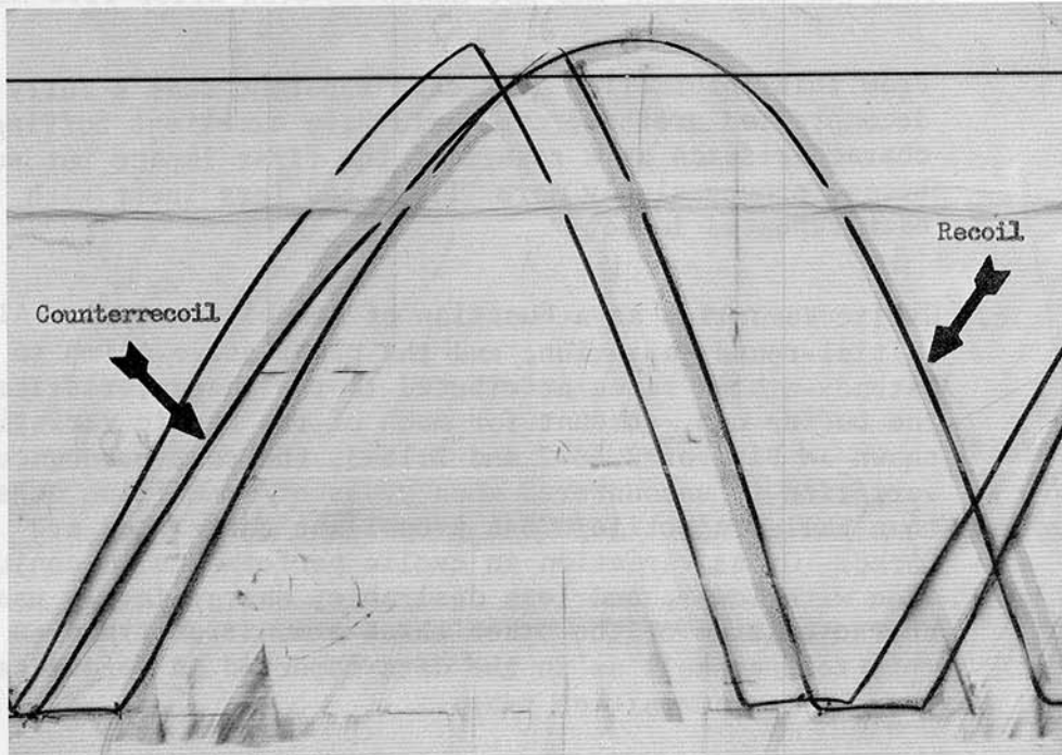
Figure 2.16-4: Displacement-Time Record During Burst Fire, Lot TW18007, Record No. 6. Traces of Rounds No. 8, 1 and 16, from Left to Right, Are Shown. Arrows Indicate Trace of Round No. 1, a Short Recoil Round.
