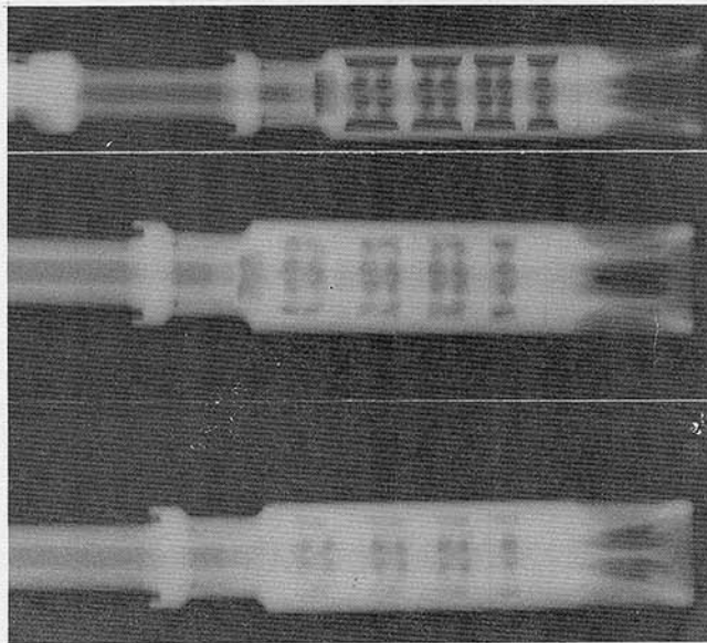
Figure 2.2-11: Flash Suppressor of XM177E2 No. 904549 before Firing and after Firing 1000 and 2064 Rounds (TOP to BOTTOM).
