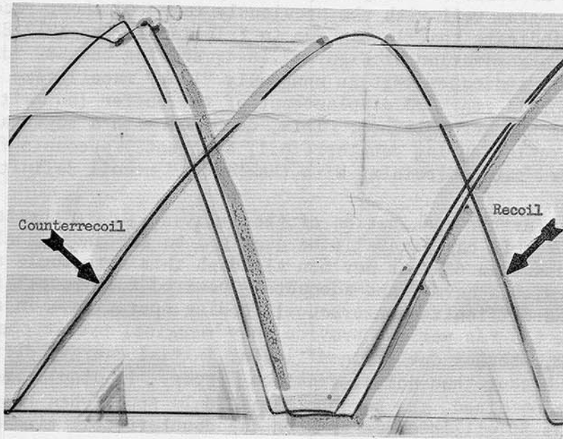
Figure 2.16-5: Displacement-Time Record During Burst Fire, Lot TW18007, Record No. 6. Traces of Rounds No. 12, 20 and 4, from Left to Right Are Shown. Arrows Indicate Trace of Round No. 4, a Short Recoil Round.
