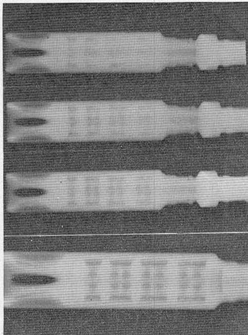
Figure 2.2-5: Flash Suppressor of XM177E1, No. 902159 after Firing 180, 1200, 2700, and 5700 Rounds (TOP to BOTTOM).
