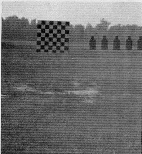
Figure I-10: Target Obscuration Effect of Smoke while Firing Semiautomatically, Ten Rounds Each of Four Lots of Ammunition in XM177E2 Submachine Gun. UPPER LEFT: Lot LC-12081 (Tracer Projectile, Ball Propellant). UPPER RIGHT: Lot TW-18007 (Tracer Projectile, 8208M Propellant). LOWER LEFT: Lot LC-12194 (Ball Projectile, Ball Propellant). LOWER RIGHT: Lot TW-18191 (Ball Projectile, 8208M Propellant).
