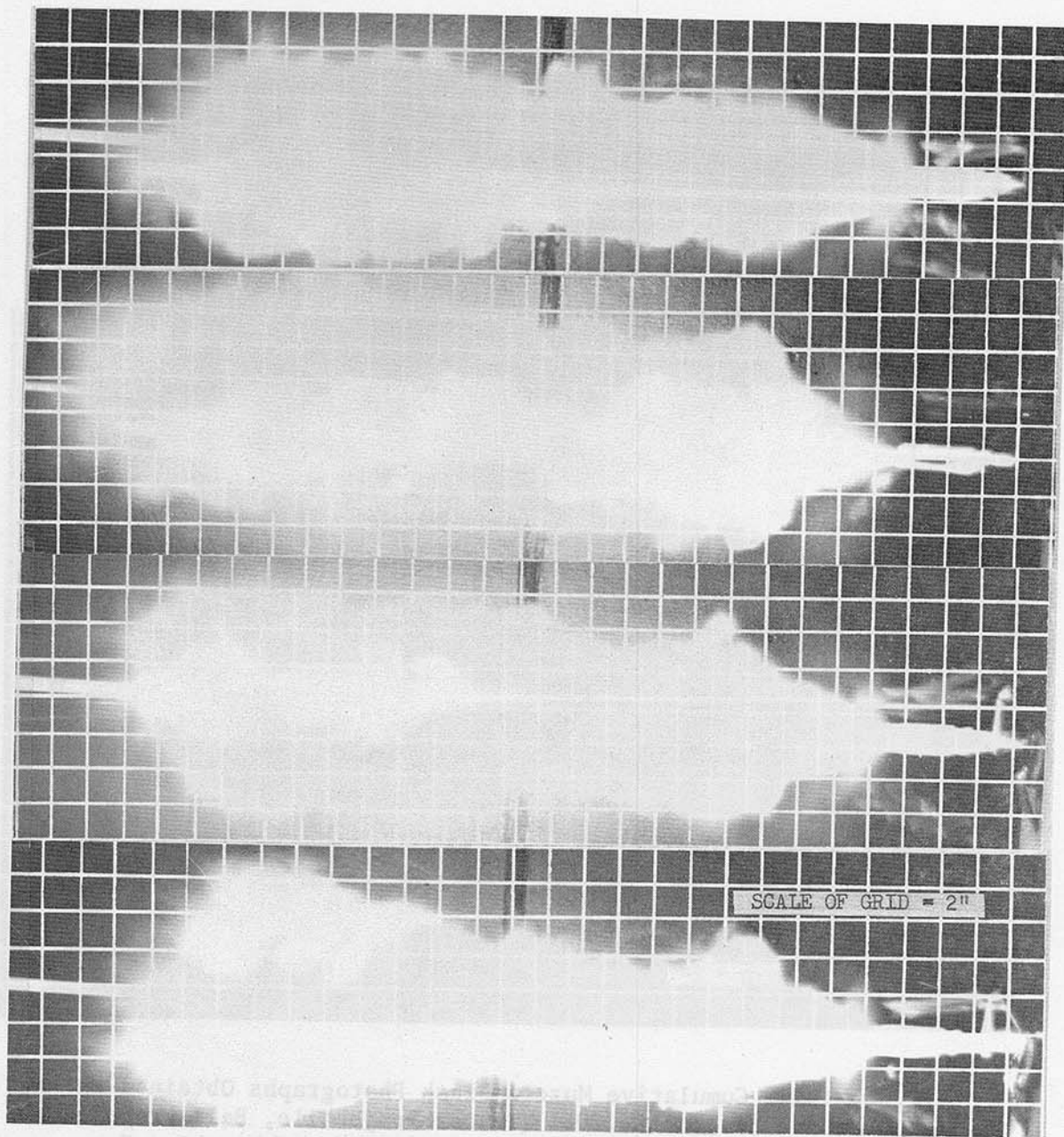
Figure I-2: Cumulative Muzzle Flash Photographs Obtained while Firing 30 Rounds of Lot LC-12081 (Tracer Projectile, Ball Propellant) in a Used Condition (Fired More than 4300 Rounds) XM177E2 Submachine Gun. TOP TO BOTTOM: Fired Semiautomatically from Cold Barrel; Semi-automatically from Preheated Barrel (Heated First by Firing 60 Rounds); Automatically from Cold Barrel; Automatically from Preheated Barrel.
