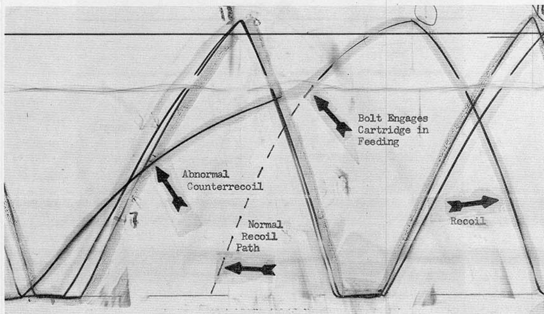
Figure 2.16-7: Displacement-Time Record During Burst Fire, Lot LC12081, Record No. 8. Traces of Rounds No. 8, 17, 1 and 16, from Left to Right Are Shown. Arrows Indicate Round No. 1, where A Cartridge Feeding Problem Was Overcome without a Gun Stoppage.
