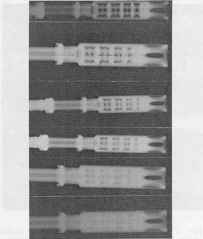
Figure 2.2-8: Flash Suppressor of XM177E2, No. 90453 before Firing and after Firing 2269, 3579, 4209, 5887, and 8887 Rounds (TOP to BOTTOM).
