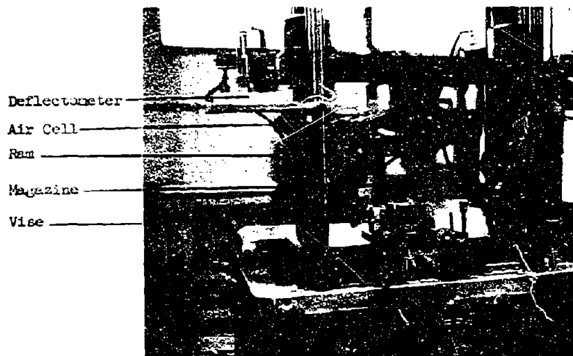
Figure I-1: Setup for Load Deflection Testing of Magazines for 5.56-201 Ammunition for M16 Rifles.
