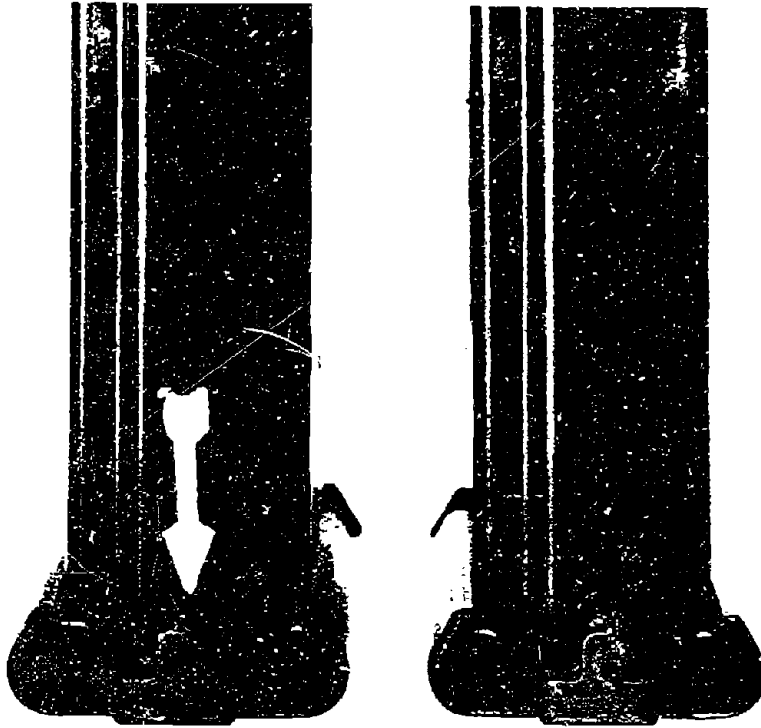
Figure 2.2-8: Rear View of the Test Magazine No. 168 Showing Irregularities of Floor Plate Latch Detent (LEFT) and a Normal Magazine (RIGHT) for Comparison.
