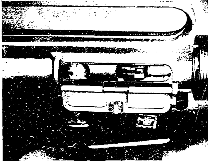
Figure 2.1-1: Right Side View of M16A1 Rifle Showing the Peculiar Type of DF Malfunction Which Occurred during This Test.
