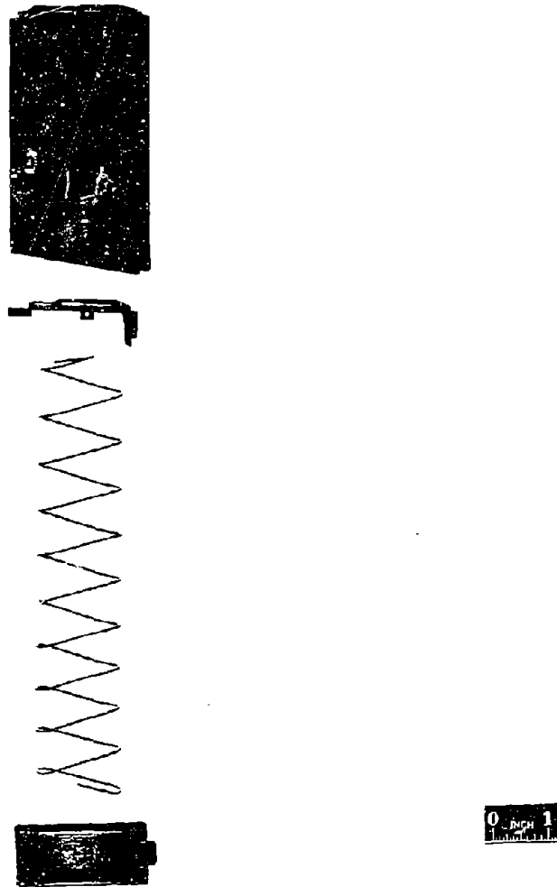
Figure 2.2-5: Disassembled View of Test Magazine (Type 1B) Showing (TOP to BOTTOM) the Magazine Body, Follower, Follower Spring, and Floor Plate.
