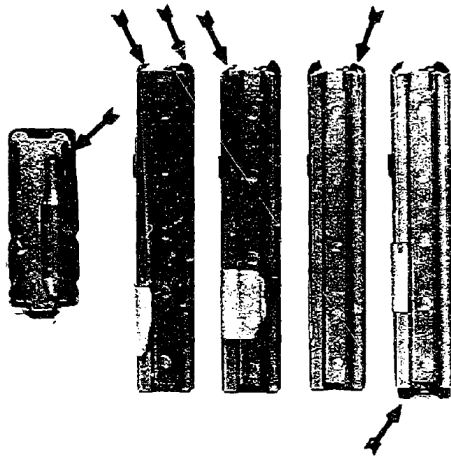
Figure 2.4-1: Five-Foot Drop Test Damage to Control Magazines at +155°F. LEFT to RIGHT: Top Forward Portion of Right Feed-Lip Bent Inward; Three Magazines with Deformed Rear Portion of Feed-Lip; and One Magazine with Floor Plate Damage. Similar Results Occurred at -65 F.
