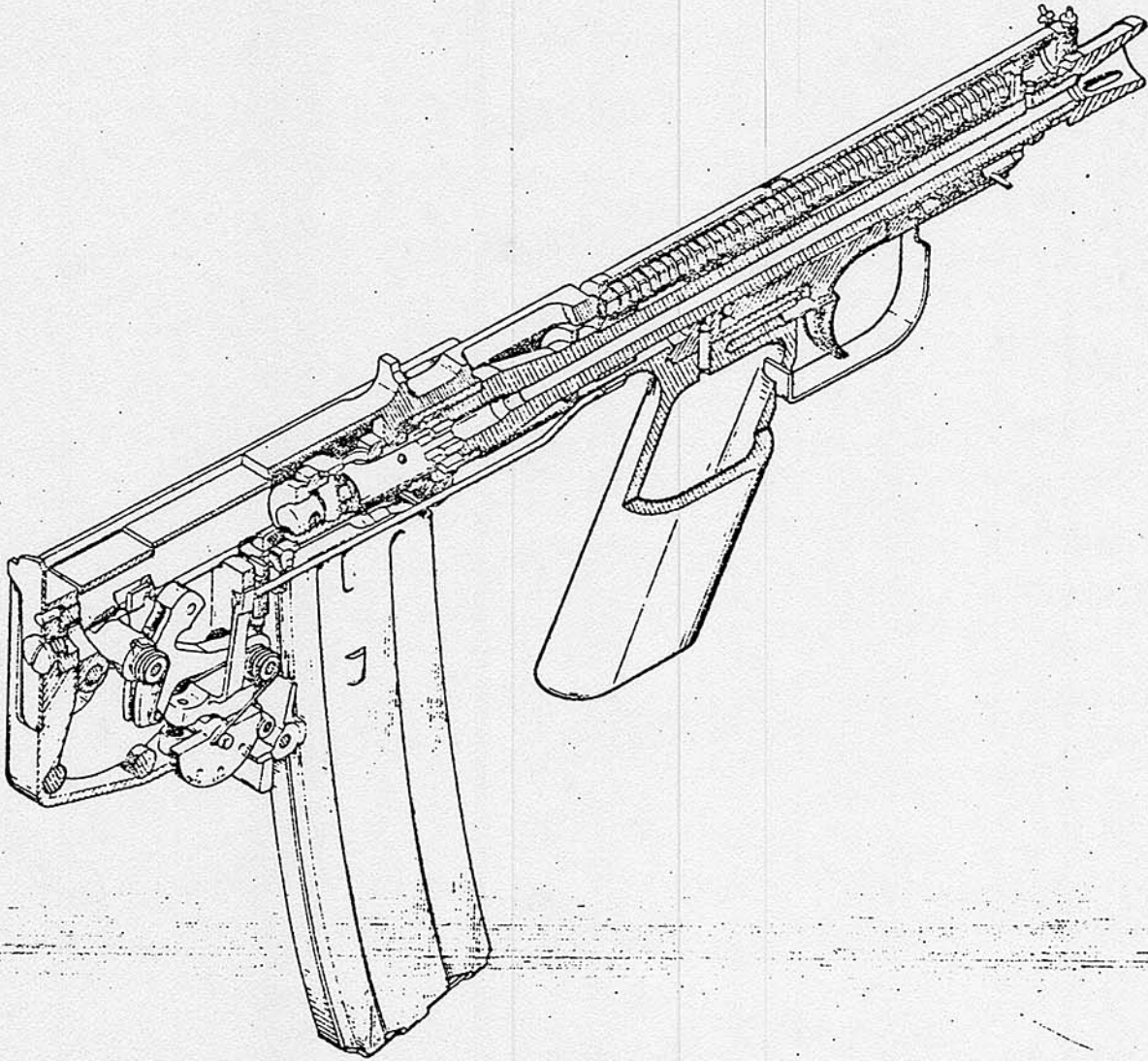
Figure 5-3. Colt's Lightweight Rifle/Submachine Gun (cutaway).
